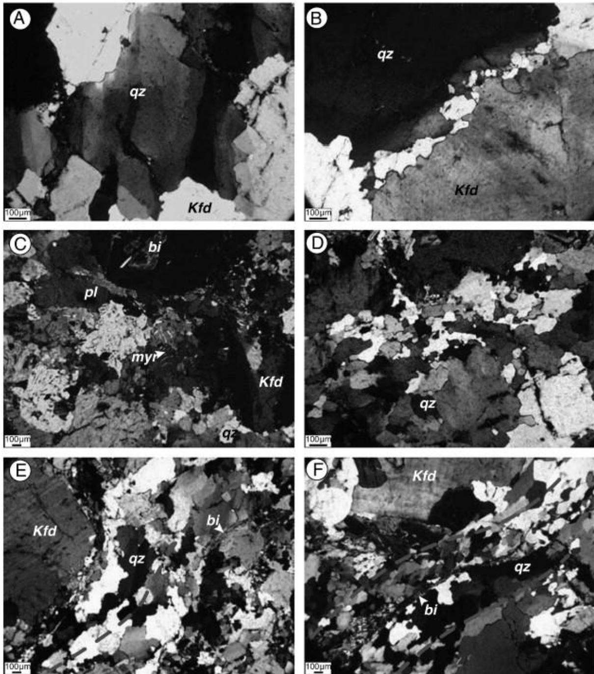
Fig. 3. Microphotographies of typical microstructures encountered within the Lüshan pluton. (A) and (B) Weak solid-state microstructures (site YU 18; E 121.74398°, N 41.6158°) with, chess-board quartz grains with undulose extinction, quartz grains with lobate borders. (C) and (D) Moderate solid-state microstructures with development of myrmekites (site YU 13, E 121.71612°, N 41.55588°) and recrystallized quartz grains (site YU 19, E 121.6918°, N 41.65178). (E) and (F) Strong solid-state microstructures with biotite foliation development and intensive quartz grains recrystallization (sites YU 01, E 121.61832°; N 41.47002° and YU 08, E 121.66843°; N 41.53384°); Kfd: potassium feldspar, qz: quartz, bi: biotite, pl: plagioclase, and myr: myrmekite.
