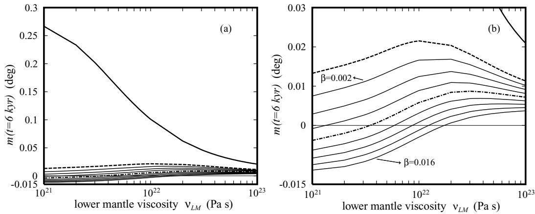
Figure 10. The present TPW displacement m(t) due to the full series of eight ice ages, evaluated at 6 kyr after the end of the deglaciation, as function of the lower mantle viscosity v_{LM} , for PREM with the elastic lithosphere (thick solid line), the high viscosity viscoelastic lithosphere, v_L = 10^{26} Pa s and with the non-hydrostatic correction \beta = 0.008 (dashed-dot line). The thin lines refer to PREM with the viscoelastic lithosphere and the non-hydrostatic correction \beta varying from 0.002 to 0.016 by steps of 0.002, from top to bottom. The negative values of m(t) indicates that the rotation pole has already crossed its initial position. The panel (b) shows the enlargement of the panel (a) in the range of [-0.015, 0.03] deg.
