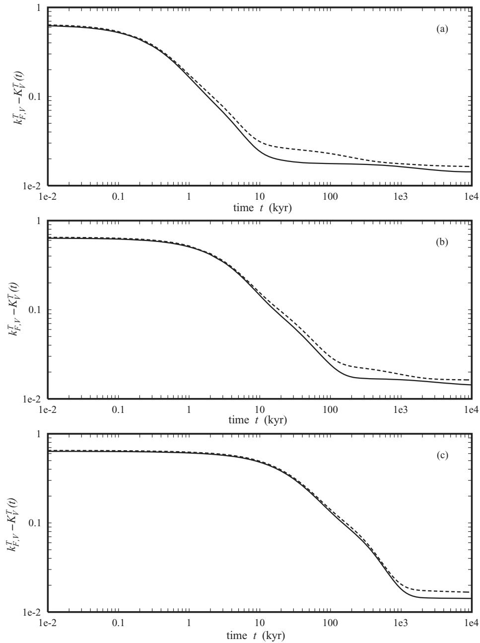
Figure 3. The readjustment of the equatorial bulge k_{F,V}^T - K_V^T(t) for the compressible (solid) and incompressible (dashed) PREM with the viscoelastic (V) lithosphere, v_L = 10^{26} Pa s. The lower mantle viscosity is v_{LM} = 10^{21} (a), v_{LM} = 10^{22} (b) and v_{LM} = 10^{23} (c) Pa s.
