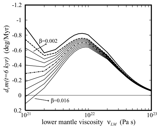
Figure 8. The present TPW rate d_m(t) due only to one ice age, evaluated at 6 kyr after the end of the deglaciation, as function of the lower mantle viscosity v_{LM} , for PREM with the elastic lithosphere (thick solid line), the high viscosity viscoelastic lithosphere, ( v_L = 10^{26} Pa s and with the non hydrostatic contribution \beta = 0.008 (dashed-dot line). The thin solid lines refer to the PREM with the highly viscous viscoelastic lithosphere and the non-hydrostatic correction \beta varying from 0.002 to 0.016 by steps of 0.002, from top to bottom. The sign of d_m(t) indicates whether the rotation pole moves forward to, negative, or go away from, positive, the Hudson bay.
