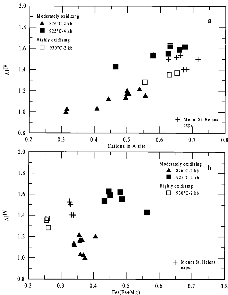
Figure 6. Compositions of experimental amphiboles (individual analyses). (a) Tetrahedral aluminium ( Al^{IV} ) versus number of cations in the A site; (b) Al^{IV} versus Fe / (Fe + Mg) , with total Fe as FeO. Amphibole compositions from the Mount St. Helens experiments at 2.0-2.2 kbar, 875-922°C, and f_{O_2} between GCH (graphite + methane) and NNO+1.2 taken from Rutherford et al. [1985] and Rutherford and Devine [1988]. Amphibole structural formulae calculated on a 23 O basis using the procedure of Richard and Clarke [1990]. Analytical errors are 2%.
