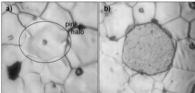
Figure 2. A halo (a) and an exfoliated area (b) observed by optical microscopy ( \times 630 ) at the surface of a sample implanted with 1 MeV helium ions at 2 \times 10^{16} ^3\text{He}^+.\text{cm}^{-2} then annealed at 1080^\circ\text{C} for 1 hour ( 100 \times 100 \mu\text{m}^2 images).
