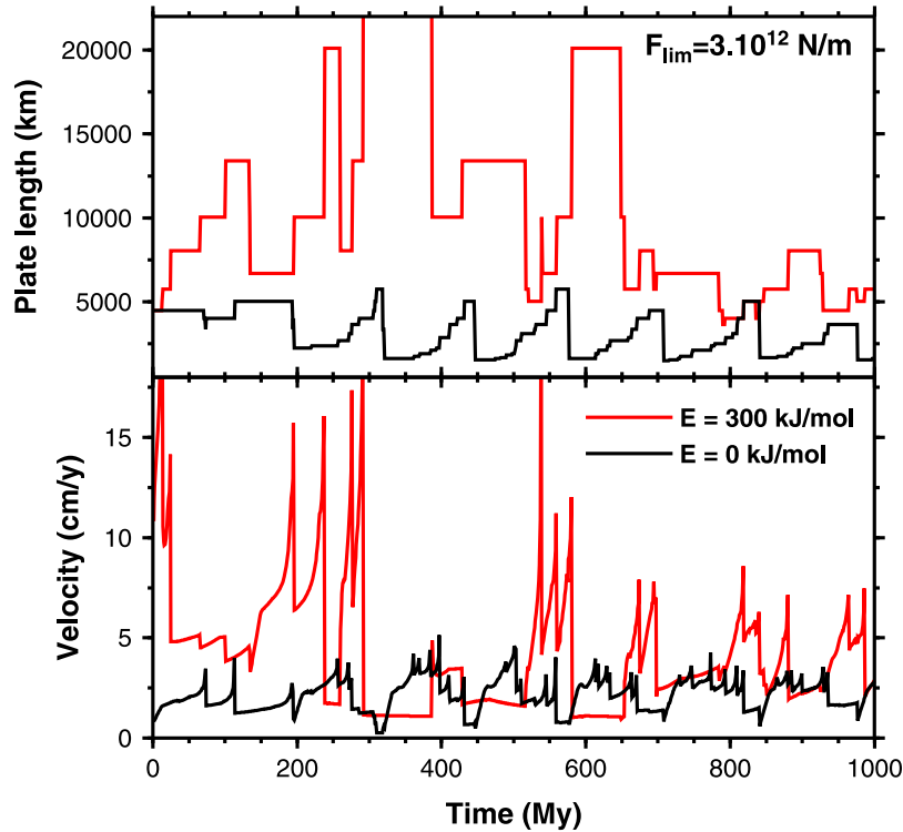
Figure 15. Evolution over 1 Gy of the average plate velocity and length for F_{lim} = 3.10^{12} \text{ N/m} and two different activation energies. Initial viscosities are respectively 3.10^{22} and 8.10^{20} \text{ Pa.s} for E = 0 and E = 300 \text{ kJ/mol} .
