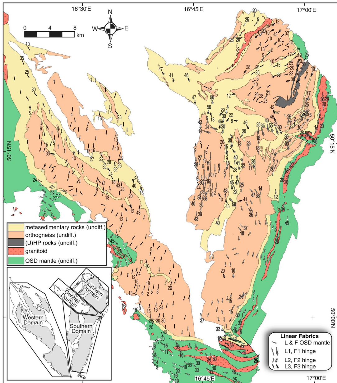
Figure 7. Structural map of linear structures (lineations and fold hinges) in the OSD. Lineations without dip are after Fajst [1976] and Příkryl et al. [1996]. Lineations in the Zábřeh and Staré Město units are after Lehmann [2009]. Inset shows the position of the different structural domains.
