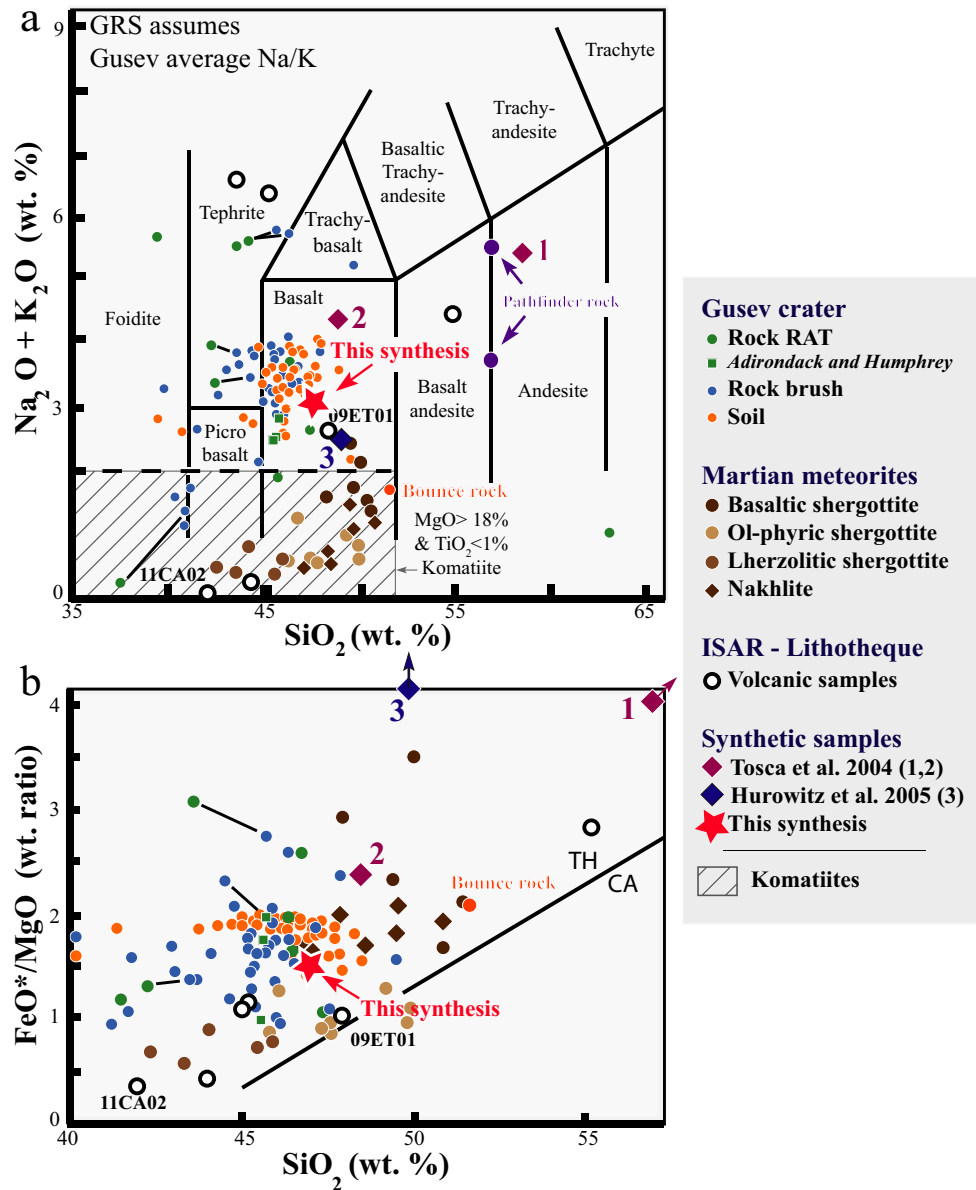
Fig. 1. Na 2 O + K 2 O oxides and FeO*/MgO ratios versus SiO 2 plots (in wt%; a and b, respectively): composition of our synthetic basalt (red star) as compared to that of in situ Martian basalts and SNC Martian meteorites (after McSween et al. 2009; Le Bas 2000). The terrestrial volcanic samples presently included in the ISAR lithotheque are also shown (black circles; sample names after Bost et al. 2011). The synthetic Pathfinder rock (1) and soil (2) from Tosca et al. (2004) and the synthetic Los Angeles sample (3) from Hurowitz et al. (2005) are also shown for comparison. The Bounce rock is the only sample of basaltic origin that was analyzed in the Meridiani Planum by the Opportunity rover (Rieder et al. 2004; Zipfel et al. 2004). The FeO*/MgO-silica diagram is used for distinguishing dry tholeiitic (TH) and wet calc-alkaline (CA) rocks. All Martian samples are tholeiitic.
