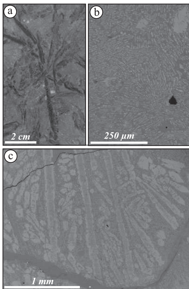
Fig. 6. Terrestrial komatiite sample from Dundonald: a) macroscopic image; b), c) backscattered images showing spinifex textures. The texture of sample 11AR01 (Fig. 3, 4) is very similar to this texture.
