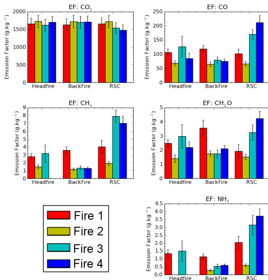
Fig. 9. Emissions factors [ \text{EF}_x ] for \text{CO}_2 , CO, \text{CH}_2\text{O} and \text{NH}_3 for the backfire, headfire and residual smouldering combustion stages (RSC) of Fires 1, 2, 3 and 4 (see Table 1 for fire details). Error bars provide a measure of emissions factor uncertainty, derived in quadrature from the uncertainty in the relevant emission ratios and a \pm 10\% uncertainty in the assumed fuel C content. Missing values represent cases where the relevant \text{ER}_x/\text{CO}_2 measure was poorly constrained, based on a low coefficient of determination ( r^2 ) between the two relevant trace gas column amounts (See Figs. 7 and 8).
