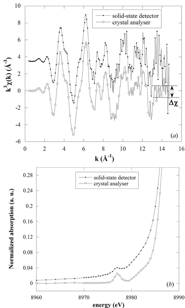
Figure 4 Comparison of k^3 -weighted EXAFS (a) and pre-edge (b) Cu K -edge spectra for a pure \alpha\text{-FeO(OH)} (goethite) containing copper (2000 ppm). Measurements were made in the fluorescence mode using a crystal analyser ( E_{\text{analyser}} = E_{K\alpha_1} , energy resolution = 1.4 eV) and 13-element Ge solid-state detector ( E_{\text{SSD}} = E_{K\alpha_{1+2}} , energy resolution = 300 eV). \Delta\chi : experimental points distribution used for the signal-to-noise ratio determination.
