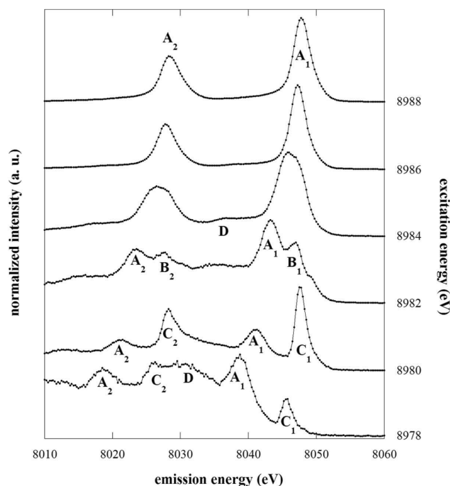
Figure 7 Emission spectra of CuO as a function of the excitation energy. Each spectrum is normalized to its maximum value.
