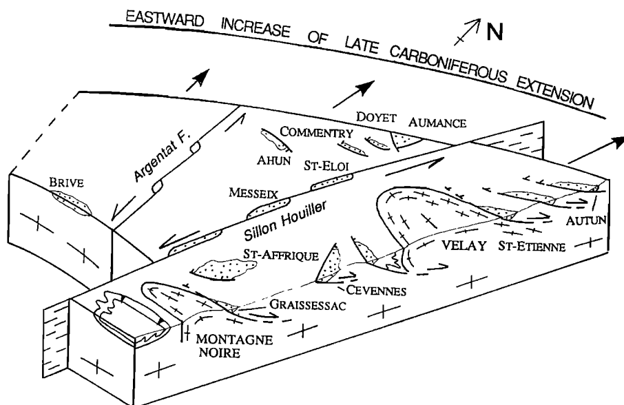
Figure 14. Schematic representation of the Late Carboniferous-Early Permian extension due to doming and basins opening. The west to east increase of extension rate is accommodated by the Sillon Houiller and Argentat fault.
