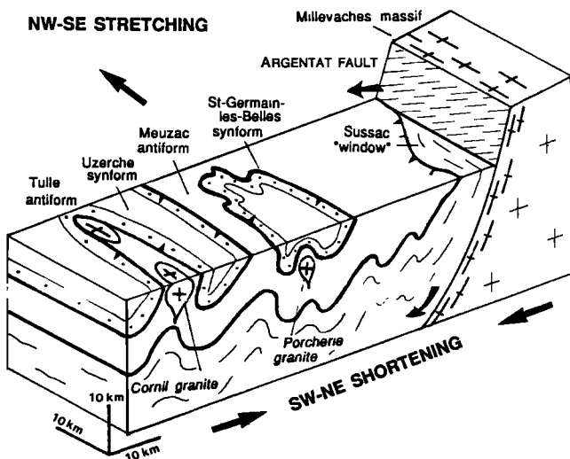
Figure 5. Schematic interpretation of the south Limousin showing the relationships between postfoliation upright folding, pluton emplacement, and normal-right lateral wrench motion along the Argentat fault.
