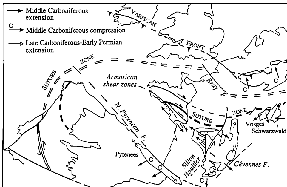
Figure 16. The two stages of extensional tectonics of the Massif Central located within the W. European Variscan Belt. Note the discrepancy in azimuth for the Late Carboniferous-Early Permian extension directions in the Massif Central and Pyrénées.
