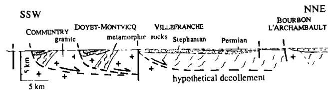
Figure 4. Structural map of the Montmarault area and cross section from Commentry to Bourbon l'Archambault showing the NE-SW extensional setting of the Late Carboniferous coal deposits. Along the Sillon Houiller, the basins are left-lateral pull-aparts, west of the Sillon Houiller the half-graben structure predominates. Commentry, Doyet-Montvicq, and Villefranche basins opened upon metamorphic basement and the Middle Carboniferous Montmarault granite which experienced a synemplacement ductile deformation. A ductile detachment fault is assumed at depth. When known, foliation and lineation trends are put inside the Montmarault granite. Solid arrows indicate the sense of shear of the upper part both in the granite mylonite (south of Bourbon l'Archambault) and the host rock (west of Saint-Eloi).
