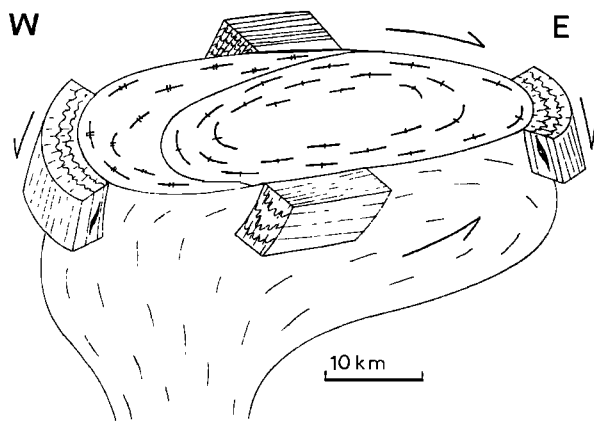
Figure 10. Inferred shape of the Cévennes plutons and their emplacement kinematics.
