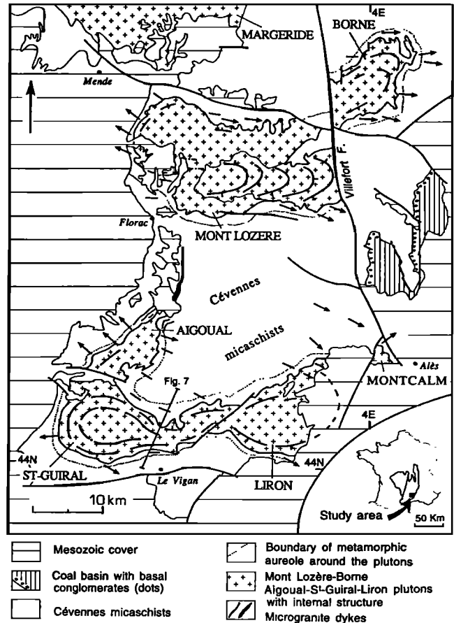
Figure 6. Structural map of the Cévennes area with emphasis of the late structures related to granite emplacement. Bar is stretching lineation related to pluton emplacement; arrows indicate the sense of shear of the upper part, both in the granite and the host rock.
