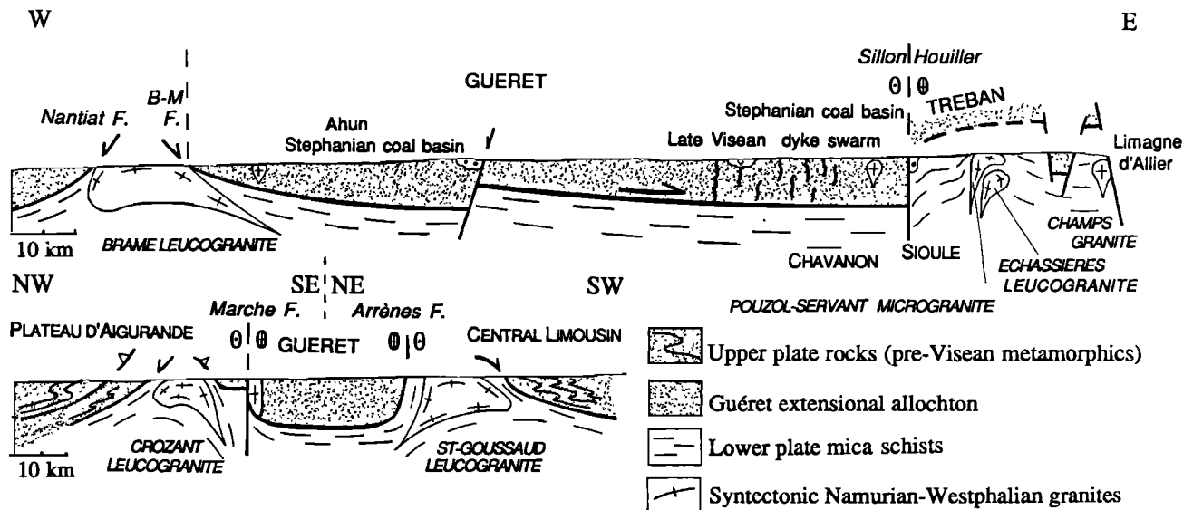
Figure 3. Cross sections through the Guéret extensional allochthon.
