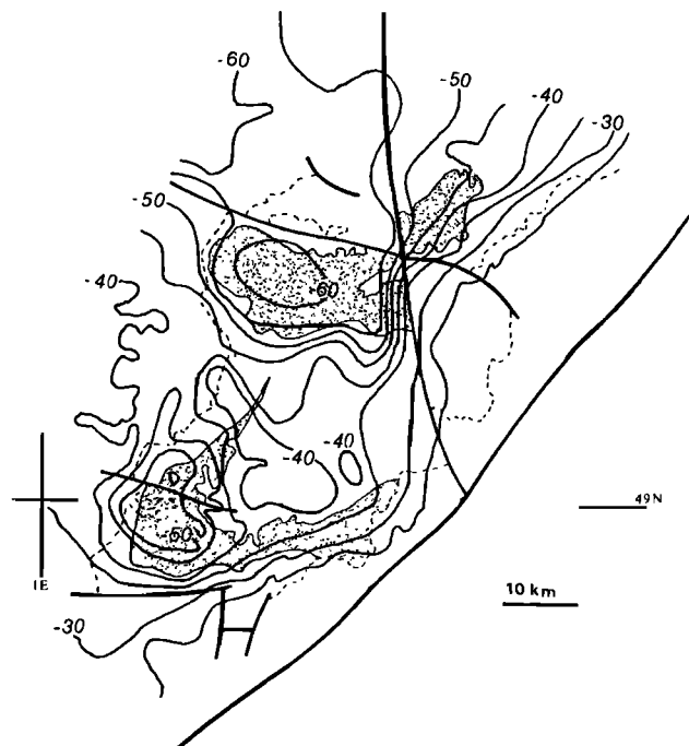
Figure 9. Bouguer gravity anomaly map of the Cévennes area. Dashed line is the the boundary of the Mesozoic cover. Note that the minima (in mGal) are located in the western part of the two plutons.
