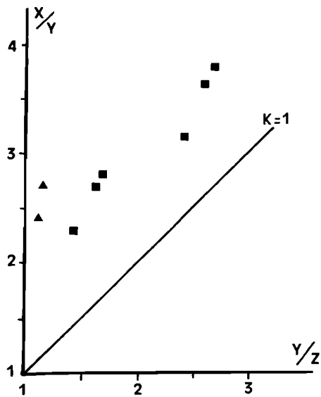
Figure 8. Flinn diagram showing the prolate shape of the mafic xenoliths. Triangles are Mont Lozère; squares are Aigoual-Saint Guiral massifs measured by J.F Babinault and I. Lucas.
