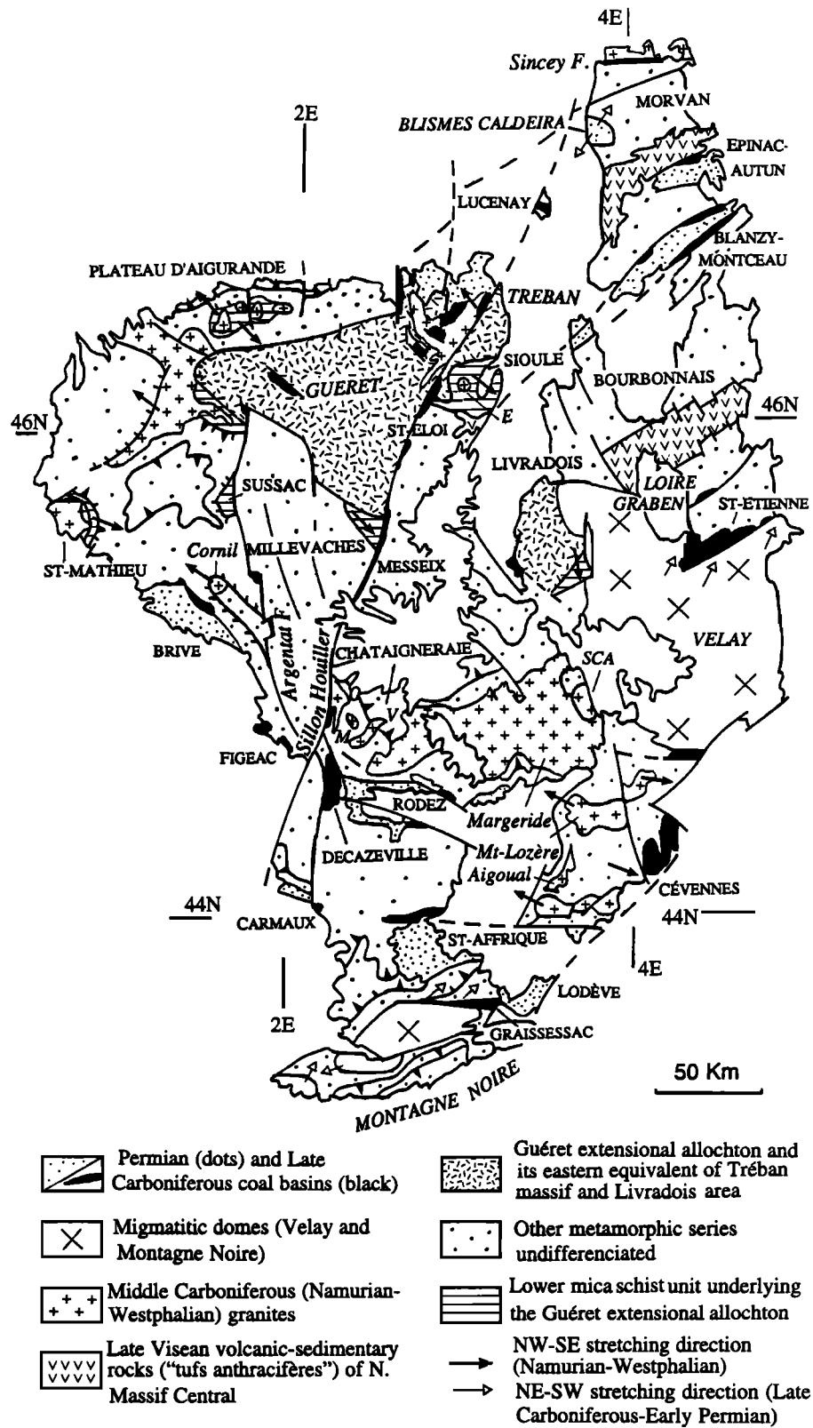
Figure 1. General map of the French Massif Central with emphasis on the Carboniferous extensional structures. Abbreviations are E, Echassières; SCA, Saintt Christophe d'Allier; V, Veinazès; and M, Marcolès.
