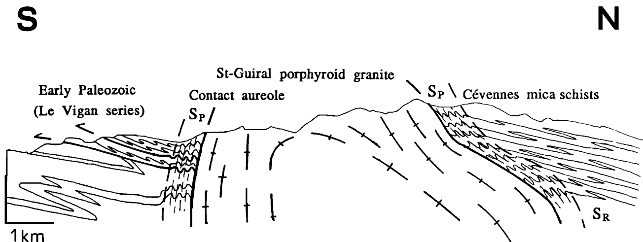
Figure 7. Cross section through the Saint Guiral granite (adapted from work of Arthaud as discussed by Alabouvette [1988]). S_R is regional foliation in the Cévennes mica schists; S_P is pluton-related foliation in the contact auréole.
