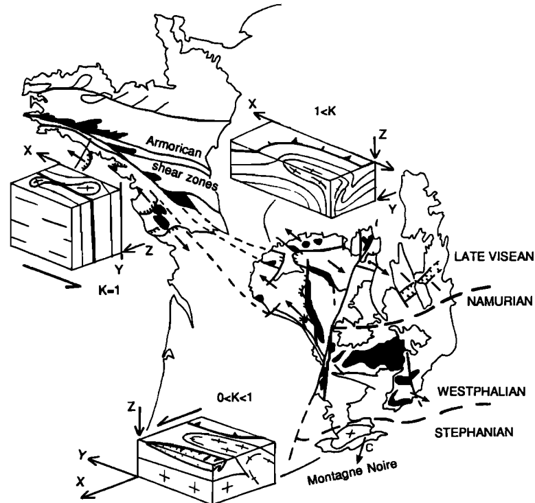
Figure 15. Relationships between wrench, extension, and compression in the southern Armorican-Massif Central branch of the Variscan belt. Late Visean, Namurian, Westphalian, and Stephanian correspond to the age of beginning of extension which is shifted to the south with time. Solid areas are the main Carboniferous plutons used as crustal strain markers. Bar indicates the stretching direction; arrows show the sense of shear of the upper part.
