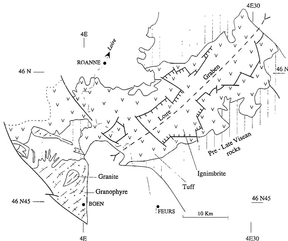
Figure 12. Late Visean extensional setting of the ignimbrite and tuff formations (Tufs anthracifères) in the Loire graben (adapted from Leistel and Gagny [1984] ).
