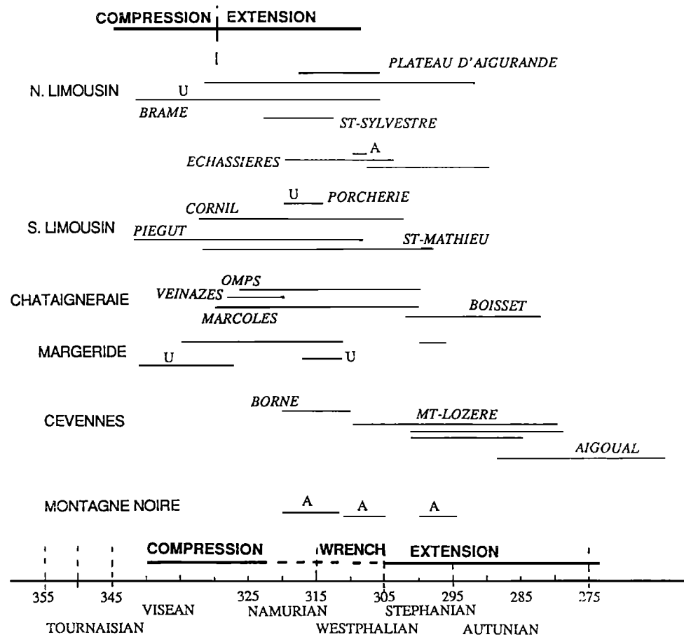
Figure 13. Timing of granite emplacement in the Massif Central in relation with the N. to S. migration of stress fields. A and U stand for ^{40}\text{Ar}/^{39}\text{Ar} and U/Pb methods, respectively; others are Rb/Sr ages recalculated with \lambda = 1.42 \cdot 10^{-11} \text{ year}^{-1} (references in the text).
