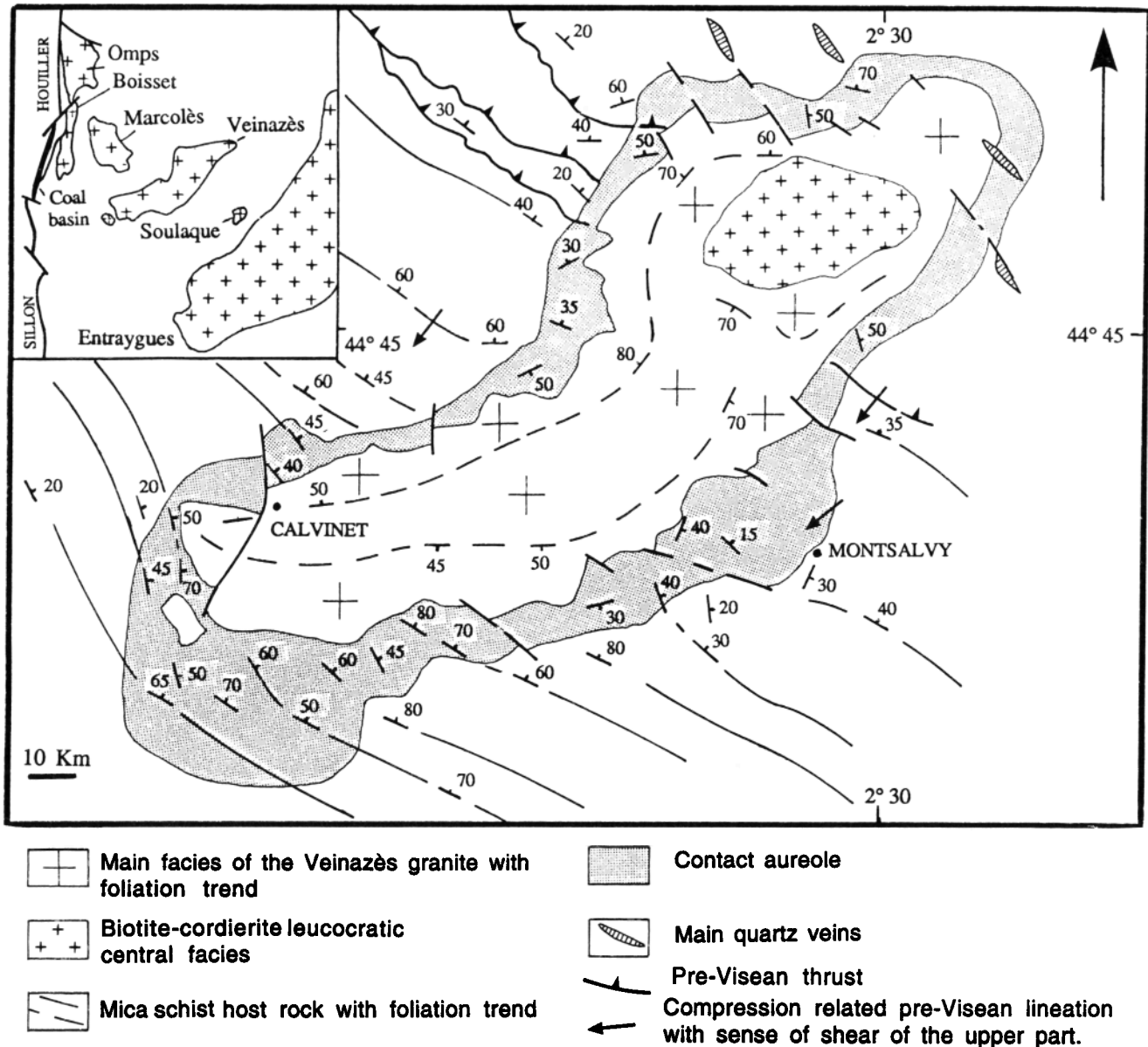
Figure 11. Structural map of the Veinazès pluton in the Châtaigneraie area showing its crustal scale "tension gash" shape, mapped with the collaboration of A. Chauvet.
