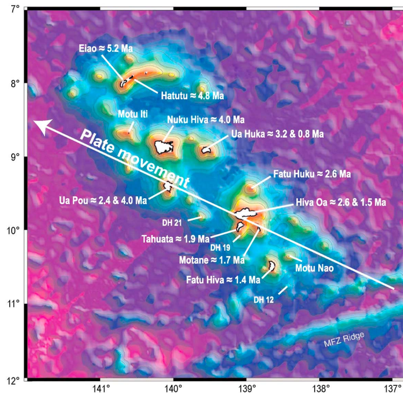
Figure 1. Location map of Marquesas Islands. The bathymetry comes from the global altimetry data set of Smith and Sandwell [1997]. Shades of purple denote depths of 5,000 to 4,000 m; shades of blue, depths of 4,000 to 2,000 m and shades of orange, depths less than 2,000 m. The main trend of the Marquesas chain is N40°W. Current Pacific plate motion is 10.5 cm/yr at N65°W, corresponding to the line shown in white and labeled plate movement. This line is also the line separating the two groups of islands as shown in Figures 4 and 5. In Hiva Oa, the line is located on the south-western side of the island in the Taaoa Bay (see Figure S1 for more details). MFZ: Marquesas Fracture Zone.
