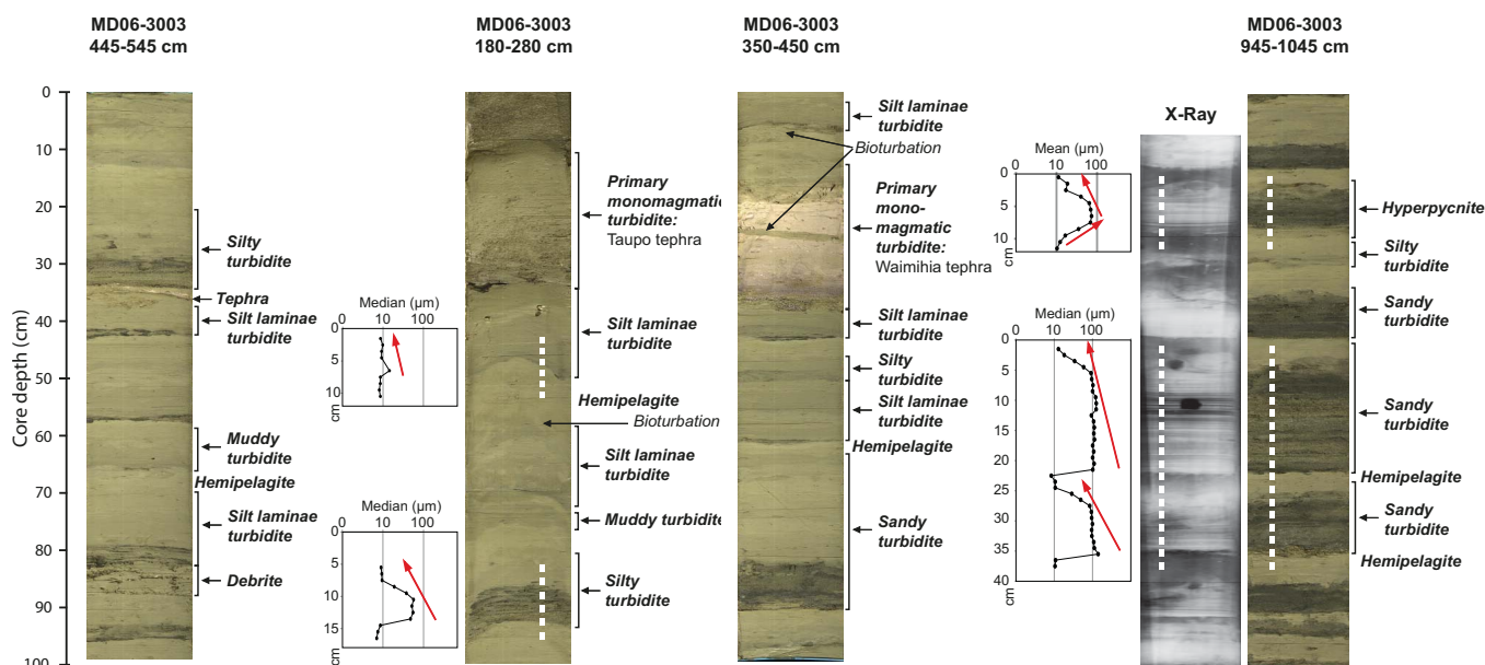
Fig. 3. Main lithofacies identified in cores from high resolution photos, grain size analysis and X-ray: hemipelagite, tephra, turbidite and debris flow (from Pouderoux et al., 2012). Grain-size data are presented for some turbidites (either the median or the mean values). Samples are taken at <1 cm intervals; position of samples is indicated by dashed lines on photos.
