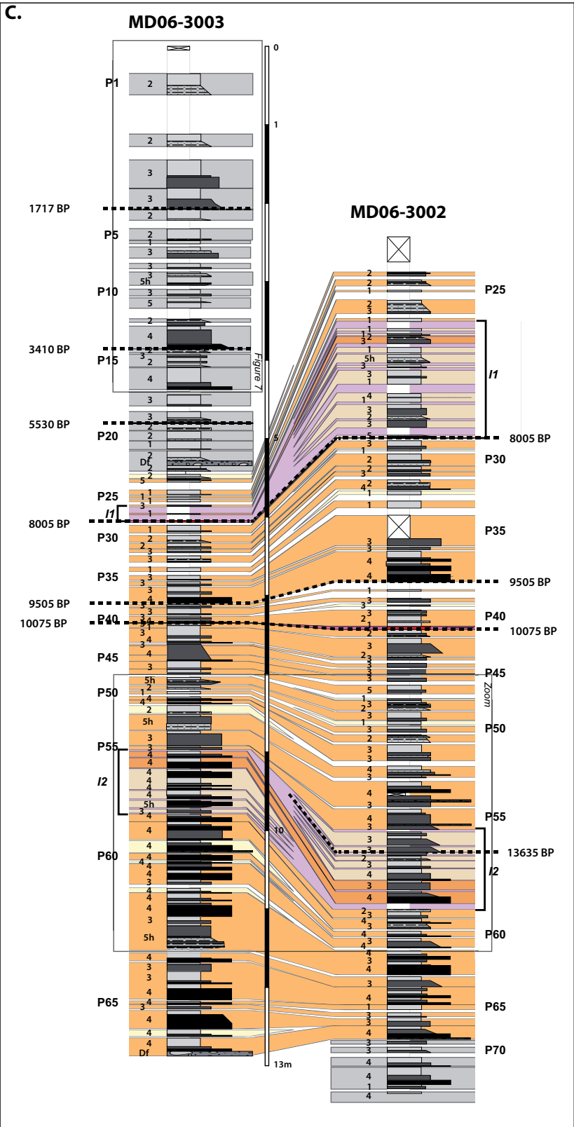
Fig. 5. (C) Turbidite correlation between cores MD06-3002 and MD06-3003, showing the high proportion of basin events and the two short intervals Int1 and Int2 of irregular turbidite deposition. Dashed lines are time markers from tephras.
