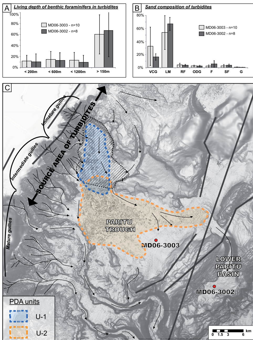
Fig. 6. (A) Turbidite content of benthic foraminifers in a selection of turbidites in both cores ( n = number of sampled turbidites, \sim 10\% of the total number). Foraminifers have been arranged in four categories following their living depth (Poudoux et al., 2012). (B) Turbidite sand composition for the same samples as in A. Sand grains are divided in seven categories: VCG: volcanoclastic grains, LM: light minerals, RF: rock fragments, ODG: other detritic grains, F: foraminifers, SF: shell fragments, G: glauconite. (C) Bathymetry of the Paritu Turbidite System showing sediment pathways (black arrows), earthquake source active faults (grey lines), cores (red dots), and the estimated source area for turbidites (gullies from Mountjoy and Micallef, 2012).
