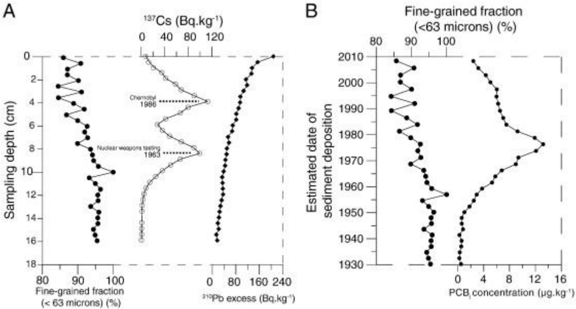
Fig. S-6. Grain size and radionuclide data by depth (A) and grain size and PCB i profiles by date (B) for a sediment core from Lake Paladru (PAL), Rhône basin, France.
