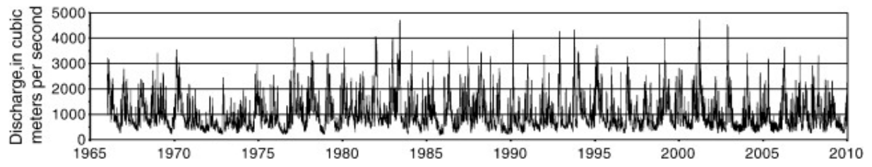
Fig. S-1. Rhône River daily mean discharge, as measured at the streamflow-gaging station at Ternay, near the city of Lyon
