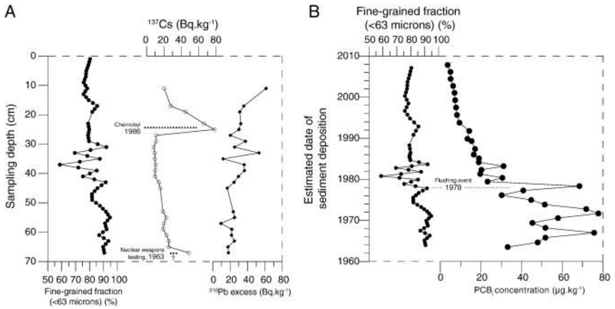
Fig. S-7. Grain size and radionuclide data by depth (A) and grain size and PCB 1 profiles by date (B) for the sediment core from La Morte (MTE), Rhône basin, France.
