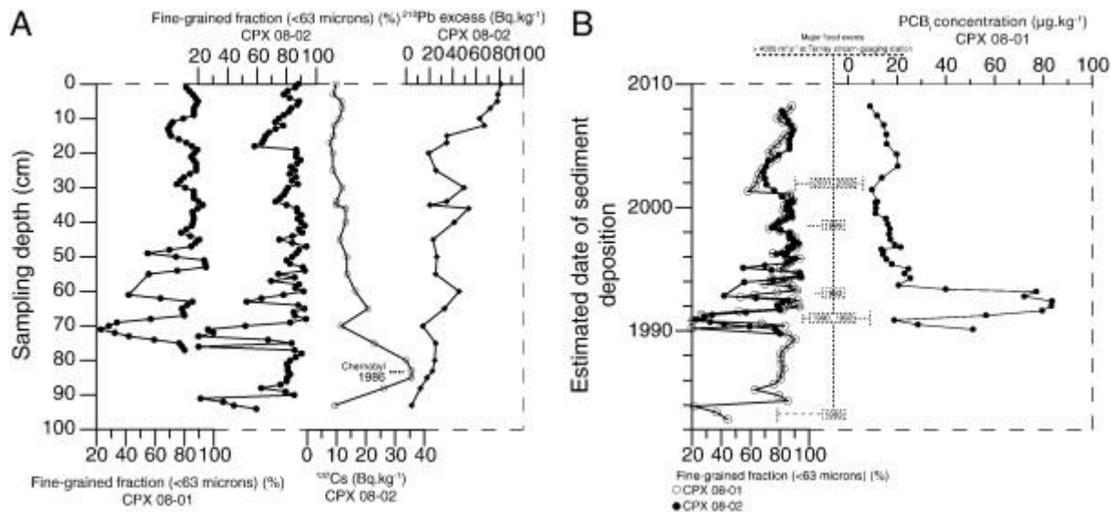
Fig. S-8. Grain size and radionuclide data by depth (A) and grain size and PCB 1 profiles by date (B) for primary (CPX 08-01) and radionuclide (CPX 08-02) sediment cores from Crépieux-la-Pape (CPX), Rhône basin, France.
