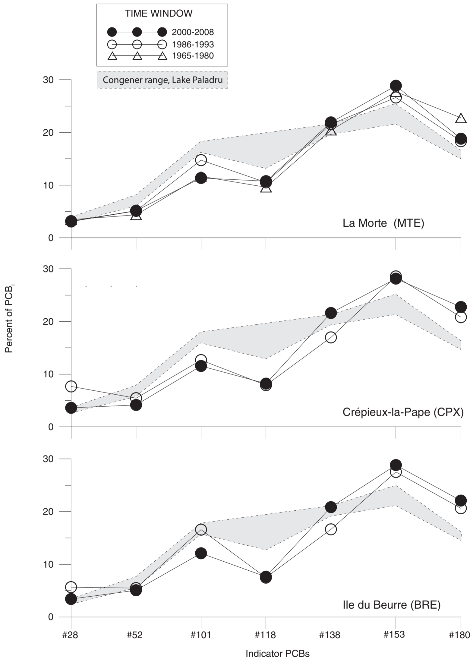
Figure 4. Profiles of the seven indicator PCBs at the three sediment coring sites along the Rhône River, France, for three time windows. Each congener is expressed as its proportional contribution the sum (PCB i ). The grey area indicates the range of profiles for the rural reference site Lake Paladru.
