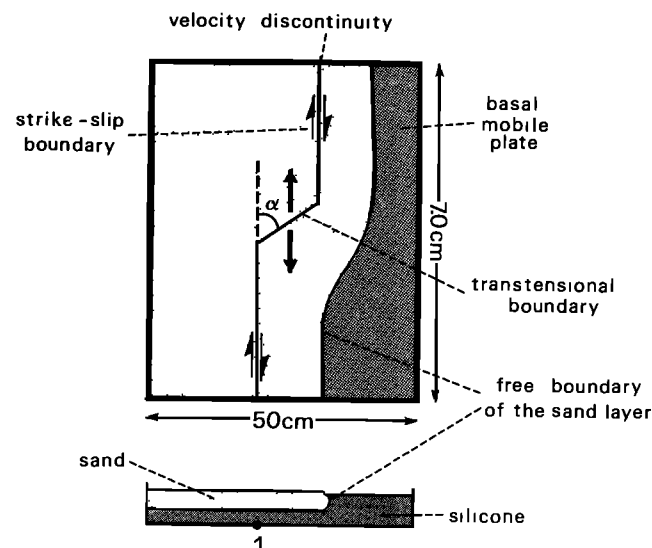
Fig. 7. Schematic description of the small-scale experiments (1 shows velocity discontinuity).
