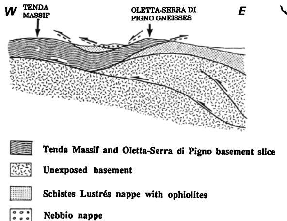
Fig. 14. E-W cross section of the Cap Corse in the Bastia area, after Warburton [1986].
