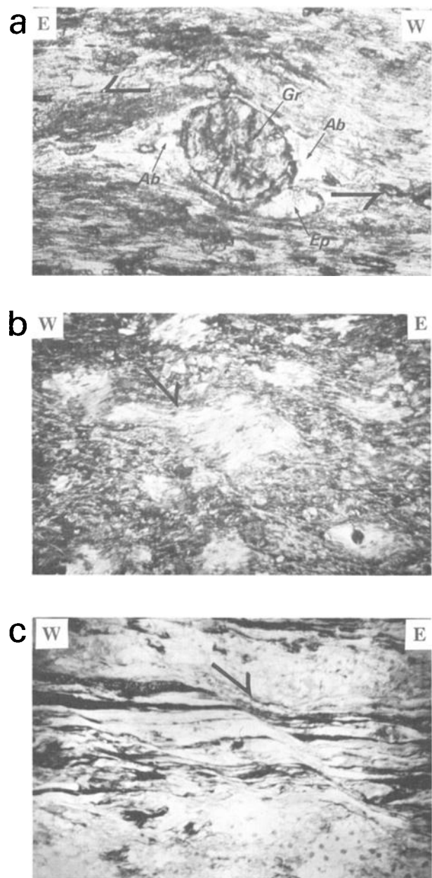
Fig. 13. Microscopic eastward shear criteria. (a) late albite crystallizing in asymmetric pressure shadows around garnet in the Lancône glaucophanites; (b) late albite crystal overprinting the earlier HP-BT foliation cut by eastward shear plane; (c) shear planes in the Cap Corse calcschist.
