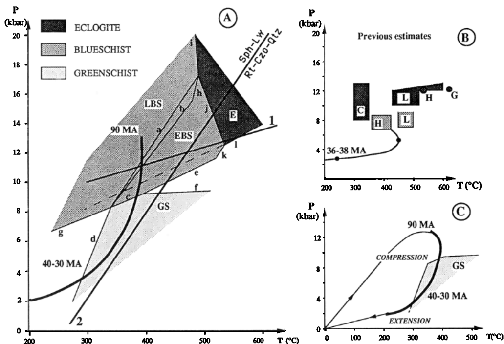
Fig. 6. P-T path in the Schistes Lustrés nappe. (a) P-T path for the Lancône glaucophanites (after calculations of Evans [1990]), E, eclogites; EBS, epidote-blueschist; GS, greenschist; LBS, lawsonite-blueschist. Reaction list (assemblages on the left are stable on the higher-pressure side): a, lawsonite (Lw) + jadeite (Jd) + tremolite (Tr) = clinozoisite (Czo) + glaucophane (Gln) + quartz (Qtz) + H 2 O (W); b, Lw + Gln = paragonite (Pg) + Czo + chlorite (Chl) + Qtz + W; c, Gln + Czo + Qtz + W = albite (Ab) + Chl + Tr; d, pumpellyite (Pmp) + Chl + Qtz = Czo + Tr + W; e, Gln + Czo + Qtz + W = Ab + Pg + Tr; f, Pg + Tr + W = Ab + Czo + Chl + Qtz; g, Lw + Gln = Pmp + Chl + Ab + Qtz + W; i, Jd + diopside (Di) + pyrope (Prp) + Qtz + W = Gln + Lws; j, Jd + Di + Prp + Qtz + W = Gln + Czo; k, Czo + Qtz = Ab + Prp + Tr + W; l, Jd + Qtz = Ab; 1, Si content of phengites = 3.47 [after Massonne and Schreyer, 1987]; 2, Sphene (Sph) + 3 Lw = Qtz + Rutile (Rt) + 2 Czo + 5 W. (b) Previous estimates for eclogites and blueschists P-T conditions: C, Caron et al. [1981]; G, Guiraud [1982]; H, Harris [1984]; L, Lahondère [1988]. P-T path for Cap Corse blueschists after Harris [1984]. (c) Synthetic P-T path for Lancône glaucophanites included in the basal ophiolitic unit. GS is greenschist.
