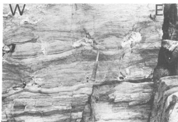
Fig. 8. Boudins of mafic sandstones metamorphosed into quartzites in the Oletta-Serra di Pigno cover (near Monte a a Torra, section b, Figure 3).
