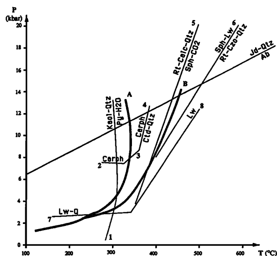
Fig. 7. Stability fields of calcschists assemblages [after Goffé et al., 1988]. A, P-T path for calcschists units; B, P-T path for schists included in the basal ophiolitic unit; 1, kaolinite (Kaol) + Qtz = pyrophyllite (Py) + H 2 O; 2, carpholite (Carph) = sudoite + Qtz; 3, Carph + Qtz = Chl + Pyr + H 2 O; 4, Carph = chloritoid (Cld) + Qtz + H 2 O; 5, Rt + calcite (Calc) + Qtz = Sph + CO 2 ; 6, Sph + 3 Lw = Rt + 2 Czo + Qtz + 5 H 2 O; 7, Lw + Qtz = laumontite; 8, Lw = zoisite + margarite + Qtz + H 2 O.
