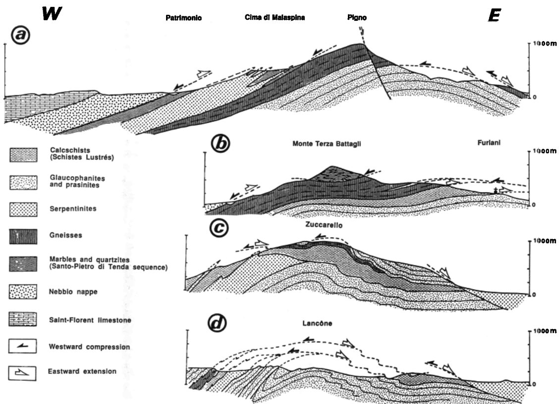
Fig. 5. E-W cross sections of the Bastia-Lancône area (see location in Figure 3). (a) Serra di Pigno cross section, (b) Monte Terza Battagli-Furiani cross section, (c) Zuccarello cross section, (d) the Lancône valley.
