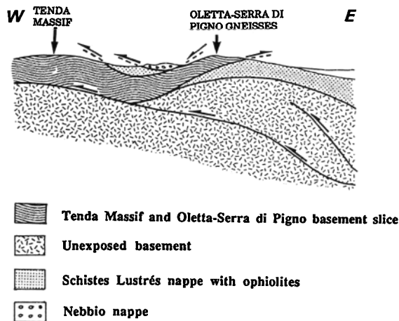
Fig. 14. E-W cross section of the Cap Corse in the Bastia area, after Warburton [1986].
