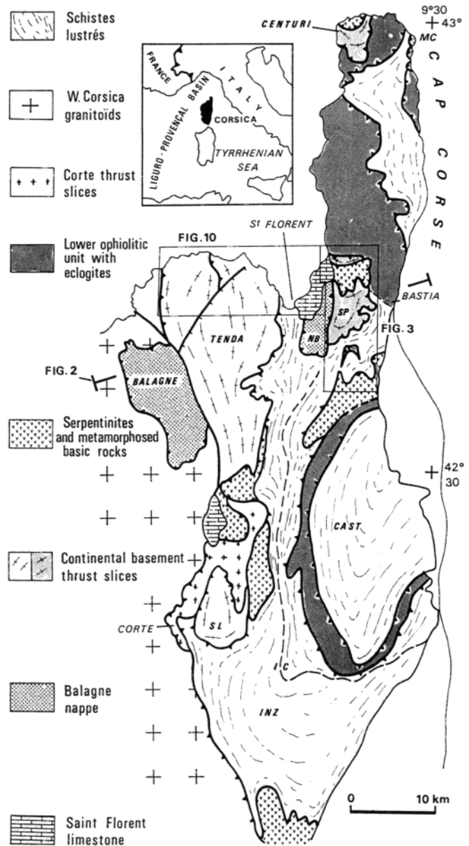
Fig. 1. Simplified tectonic map of Alpine Corsica [after Jolivet et al., 1990]. Abbreviations are CAST, Castagniccia; INZ, Inzecca; MC, Macinaggio; NB, Nebbio; SL, Santa Lucia; and SP, Serra di Pigno. The dotted line within the calcschists represents the contact between the Castagniccia (C) and the Inzecca (I) units of Caron [1977].
