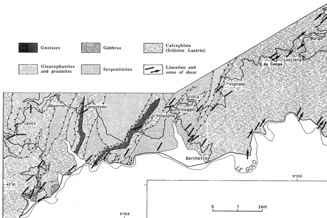
Fig. 4. Geological and structural map of the Golo valley.
