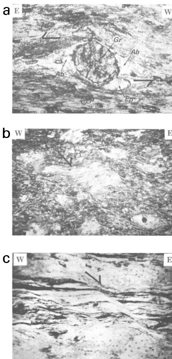
Fig. 13. Microscopic eastward shear criteria. (a) late albite crystallizing in asymmetric pressure shadows around garnet in the Lancône glaucophanites; (b) late albite crystal overprinting the earlier HP-BT foliation cut by eastward shear plane; (c) shear planes in the Cap Corse calcschist.
