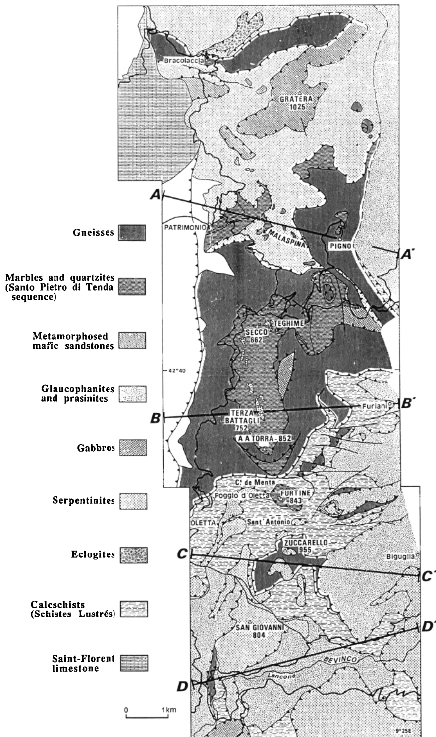
Fig. 3. Geological map of the Bastia-Lancône area.
