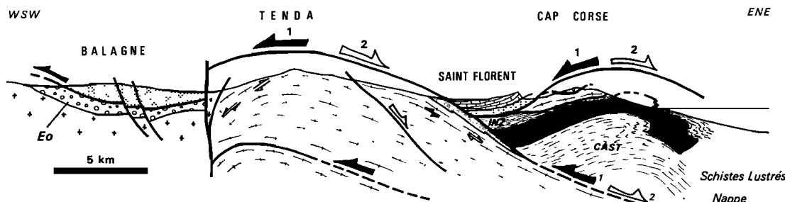
Fig. 2. Synthetic E-W cross section of the Cap Corse in the Bastia area [after Jolivet et al., 1990] (see location of the cross section in Figure 1). Solid arrows indicate the early westward compressional event (HP-LT); open arrows indicate the late eastward extensional event. For abbreviations see Figure 1. EO is Eocene autochthonous sediments.
