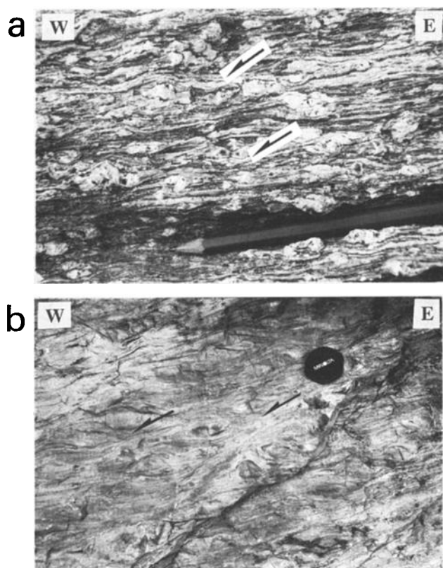
Fig. 10. C' shear planes indicating westward sense of shear in (a) the Zuccarello gneisses (section c, Figure 3) and (b) the Lancône glaucophanite (section d, Figure 3).
