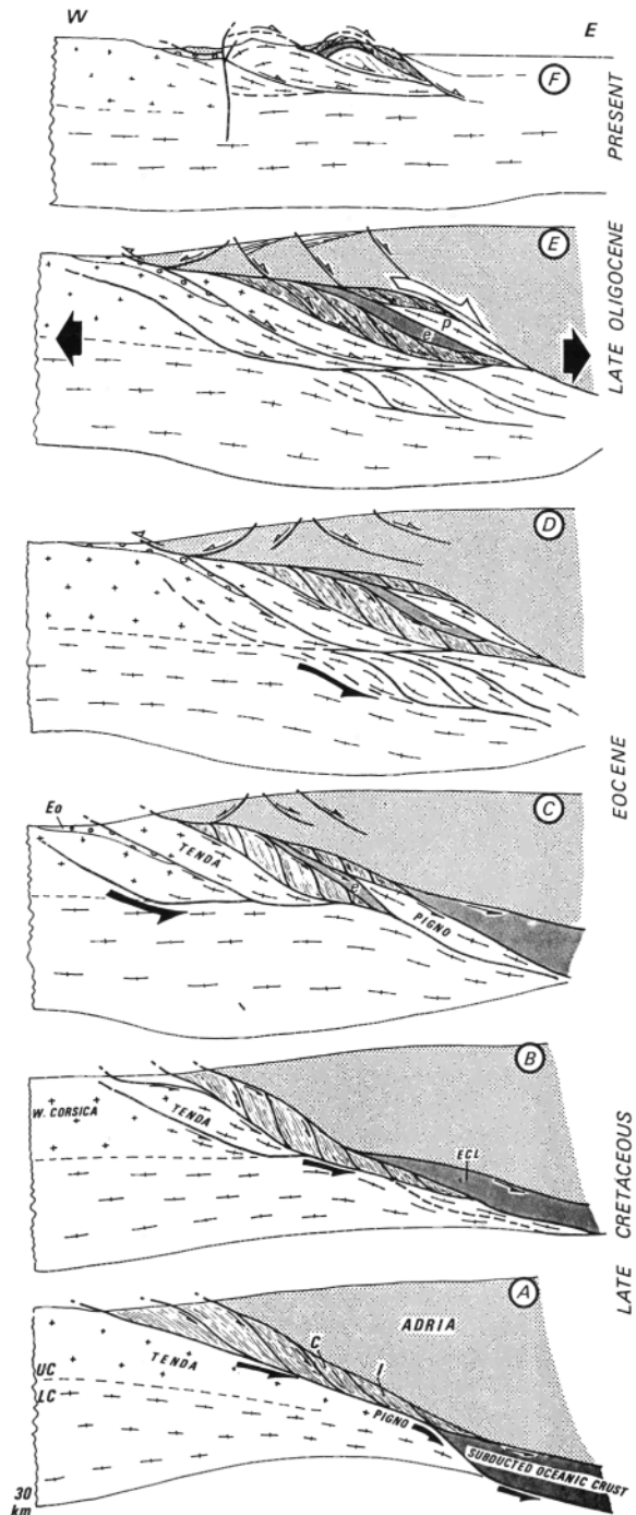
Fig. 15. Evolution scheme along the cross section of Figure 2 from the early compression in HP-LT gradient to the recent extension (explanation in text). Abbreviations are I, Inzecca, C, Castagniccia, ECL, eclogites, UC, upper crust, LC, lower crust, and eoc, eocene. (a and b), Late Cretaceous; (c and d), Eocene; (e and f), late Oligocene to Present.
