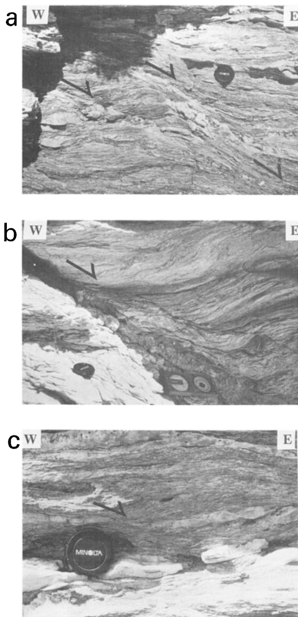
Fig. 12. Eastward shear criteria superposed along the main early thrust contacts. (a and b) Shear planes in the Paleozoic cover of the Tenda massif (west coast of the Saint-Florent gulf); (c) eastward shear plane in the Oletta-Serra di Pigno cover very near the contact with the gneisses.
