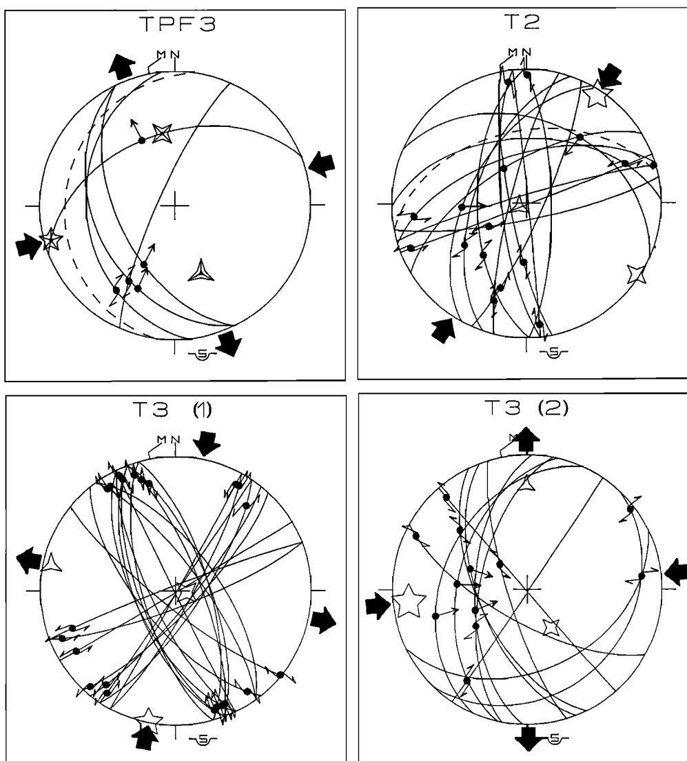
Fig. 15. Fault set stereodigraphs (lower hemisphere) and deduced paleostress field directions for sites plotted in Figure 3b. Two successive stress fields are observed on sites T3, T4, and T5.
