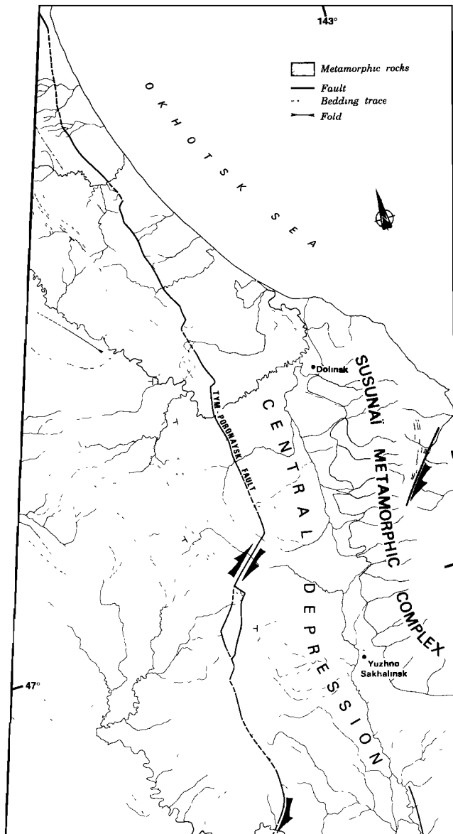
Fig. 9. Structural interpretation of a mosaic of two SPOT images of the Yuzhno-Sakhalinsk region along the Tym-Proneysk fault (localized in Figure 3c).
