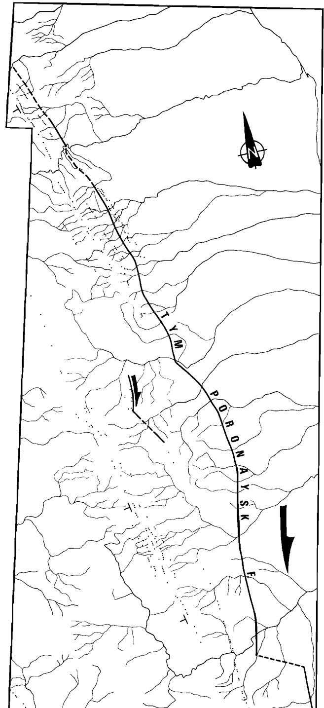
Fig. 10. Structural interpretation of a mosaic of two SPOT images along the Tym-Proneysk fault (northern region localized in Figure 3c). Same legend as figure 9. F is fault.
