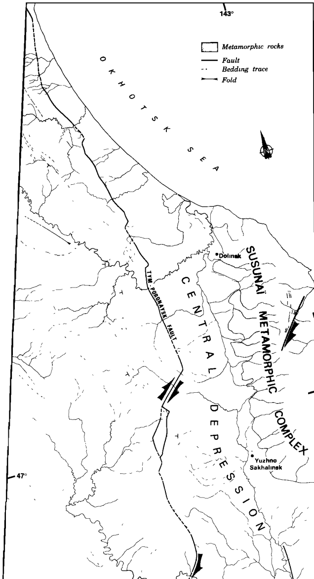
Fig. 9. Structural interpretation of a mosaic of two SPOT images of the Yuzhno-Sakhalinsk region along the Tym-Proronsk fault (localized in Figure 3c).
