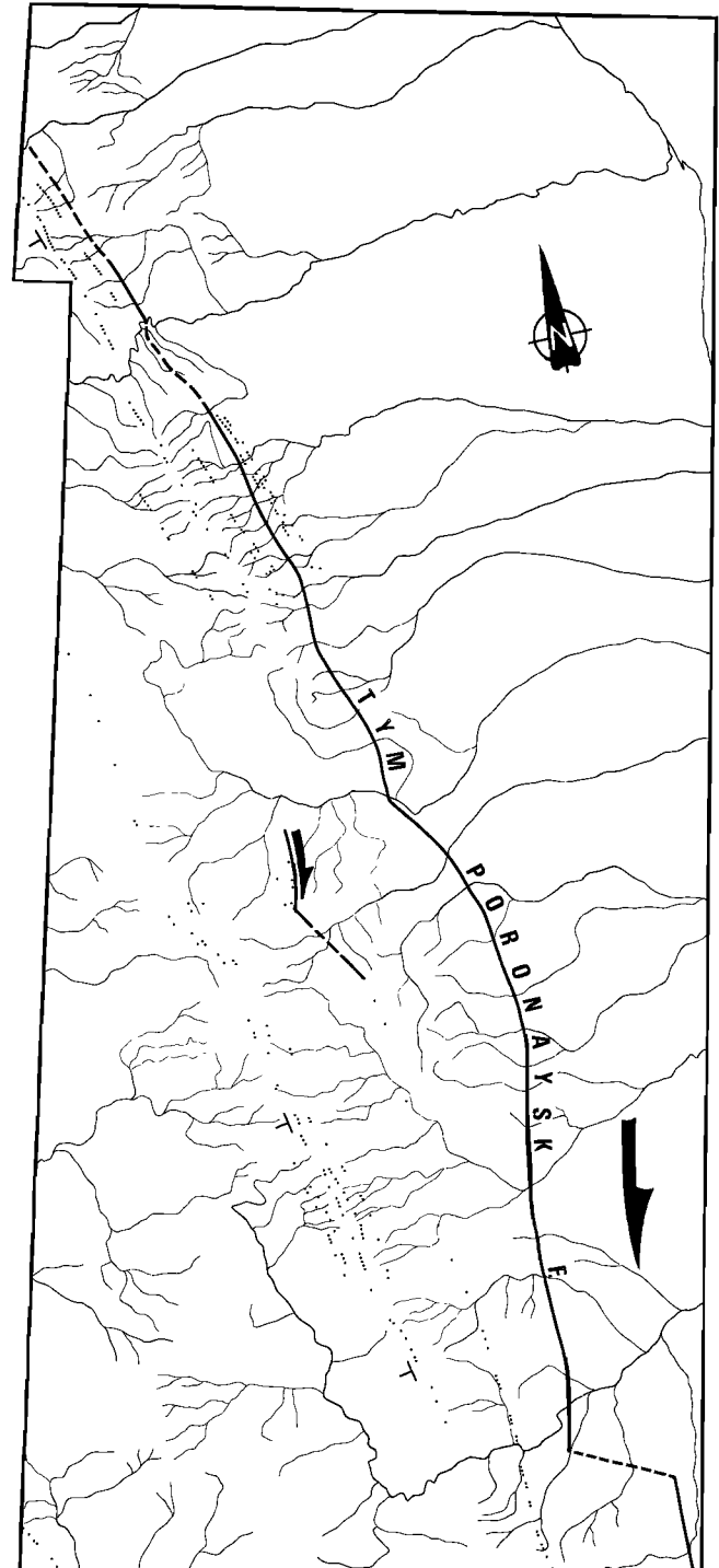
Fig. 10. Structural interpretation of a mosaic of two SPOT images along the Tym-Proronsk fault (northern region localized in Figure 3c). Same legend as figure 9. F is fault.
