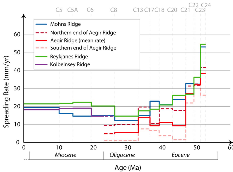
Figure 8. Spreading rates for Mohs Ridge, Aegir Ridge, Reykjanes Ridge and Kolbeinsey Ridge (Model 2). Dashed lines represent rates of spreading for northern and southern ends of Aegir Ridge.
