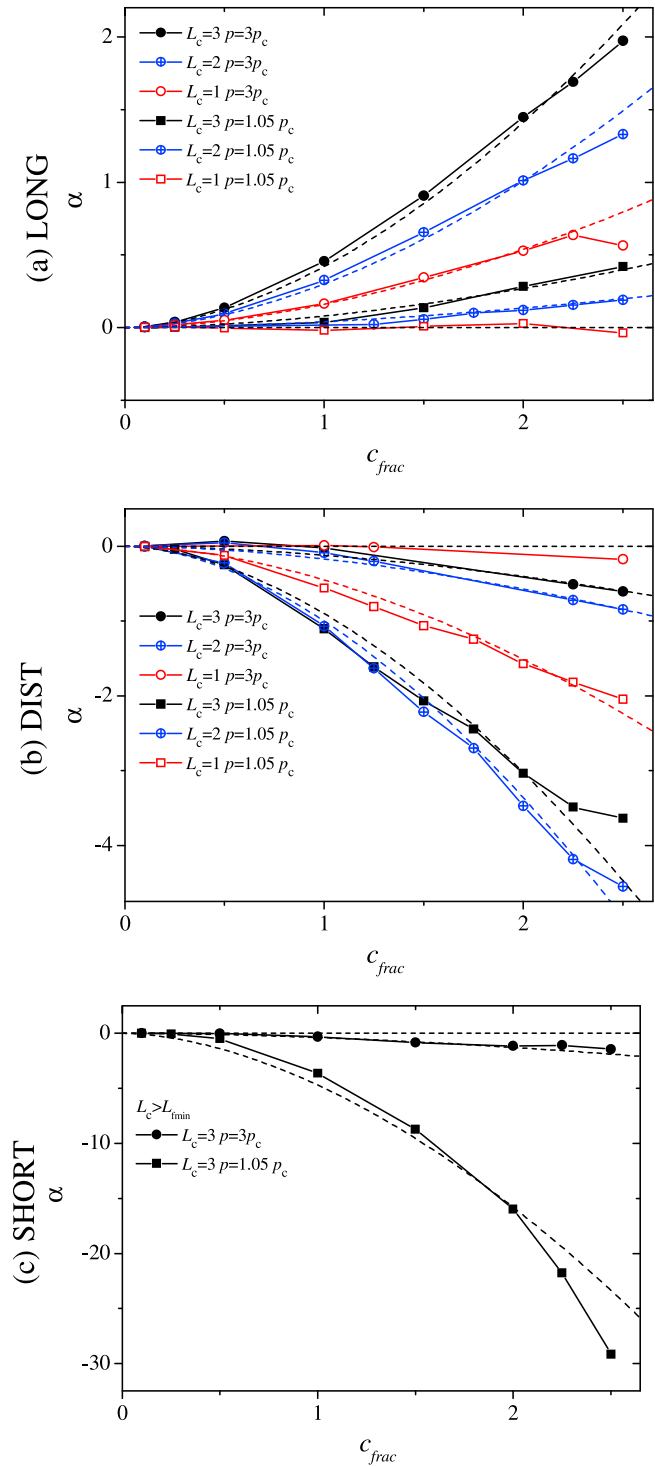
Figure 8. Permeability enhancement and reduction factors \alpha+ and \alpha- as functions of fracture closure c for different values of fracture density p/p_c and cut-off scale L_c . The dashed line next to the data plot represents the closest power law tendency: c_{frac}^{1.75} .
