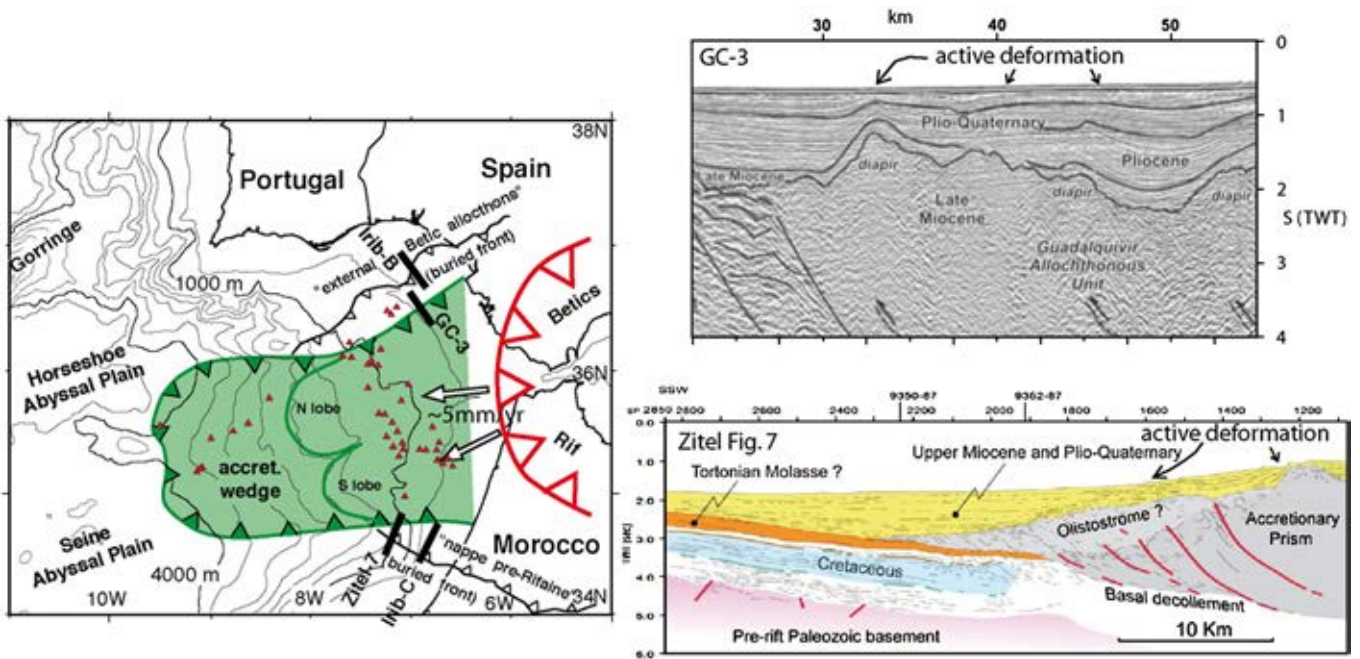
Fig. 15. Location map (left) (after Gutscher et al., 2009b) and two multi-channel seismic reflection profiles line GC-3 (upper right) (Gràcia et al., 2003b) and a Moroccan industry line (lower right) (Zitellini et al., 2009). The words “active deformation” with arrows were added.
