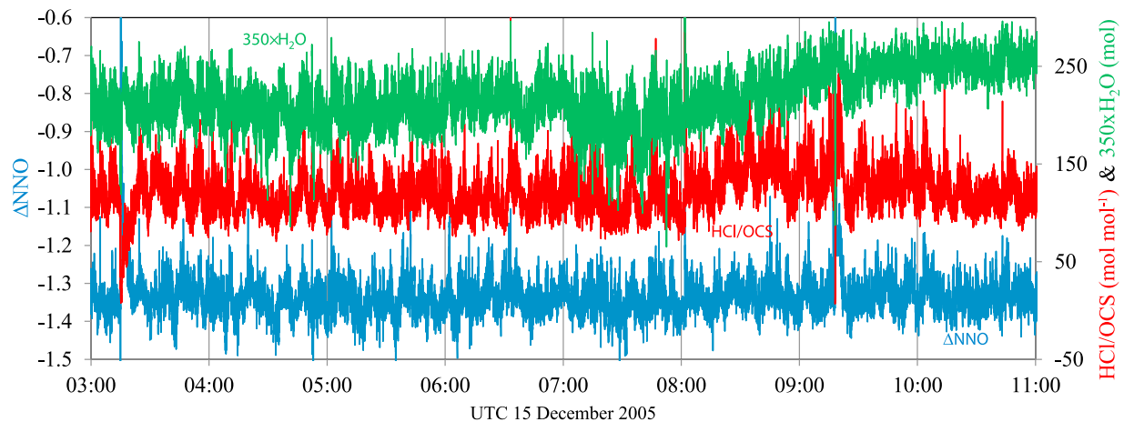
Figure 7. Eight hours on 15 December 2005 of the 1 Hz-recorded molar ratio of HCl/OCS in the gas plume emitted from the lava lake (in red), \Delta NNO in log (bar) (in blue), and the mole fraction of water in the gas plume (in green). The \Delta NNO is computed from the observed \text{CO}_2/\text{CO} ratio at 1080^\circ\text{C} . The HCl/OCS time series most clearly indicates a \sim 10 min period oscillatory behavior of the lava lake associated with the pulsed input of magma from the conduit (which is at its peak when HCl/OCS is high). The correspondence between HCl/OCS and \Delta NNO fluctuations is generally clear, indicating that the magma pulses entering the lake are about 0.1 log units more oxidized than the lava lake itself. The X_{\text{H}_2\text{O}} oscillations are also phase-locked with those exhibited by HCl/OCS and \Delta NNO, indicating that the magma pulses entering the lake are strongly degassing water at low pressure. Of note are two explosions, one at 06:15 UT, the other at 09:19, which are marked by instantaneous decrease in HCl/OCS and increase in f_{\text{O}_2} .
