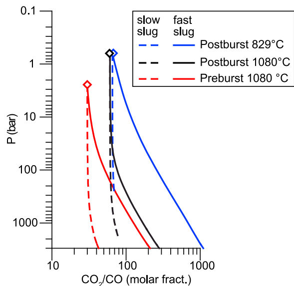
Figure 16. Evolution of \text{CO}_2/\text{CO} as a function of pressure for pre- and post-burst gas compositions. Diamonds represent three possible median compositions of the explosive gas from which isothermal backtracking is carried out. Solid and dotted lines represent fast and slow slugs, respectively.
