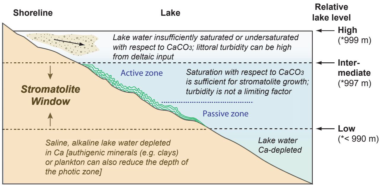
Fig. 16. Concept of the 'stromatolite window' in closed saline, alkaline lakes. Carbonate stromatolites (calcite, aragonite, dolomite or Mg-carbonates) are limited to a specific range in elevation around the shoreline that varies from lake to lake. That range is controlled mainly by the lake water chemistry (especially \text{Ca}^{2+} availability). Other factors, such as turbidity, organic productivity and its impact on the depth of the photic zone, and toxins at high salinities, can all control the vertical limits, range, thickness and morphology of stromatolite (or thrombolite) formation around the shoreline or across the lake floor. Shoreline slope controls the lateral extent of the stromatolites. In deep saline, alkaline lakes, the stromatolite window may be a restricted zone around the lake margins; in shallow lakes, however, the entire lake floor may fall within the 'stromatolite window' depending on the lake hydrochemistry and hydrology. Dilute Ca-bearing ground water seepage along lake shorelines often controls the location of the microbialites that lie within the stromatolite window.
