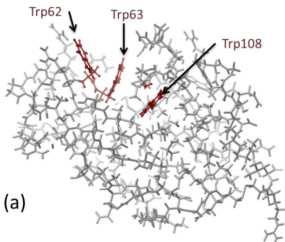
Fig. 5 Lysozyme structure (a) complete structure and (b) zoom on Trp62, Trp63 and Trp108
