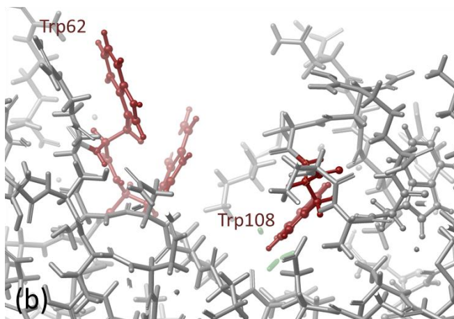
Fig. 5 Lysozyme structure (a) complete structure and (b) zoom on Trp62, Trp63 and Trp108
