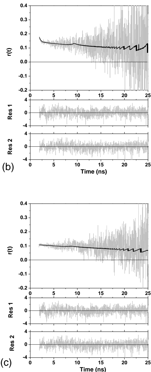
Fig.7 anisotropy decay of lysozyme loaded on (a) Na-Mt, (b) C 10 E 3 -Mt and (c) SOS-LDH (res 1 and res 2 are residues function of fit I_V(t) , I_H(t) , respectively)
