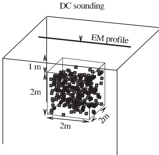
Figure 1. Heterogeneous porous medium embedded in a homogeneous half-space (hs) host-medium ( \sigma_{hs} = 0.01 S/m).
