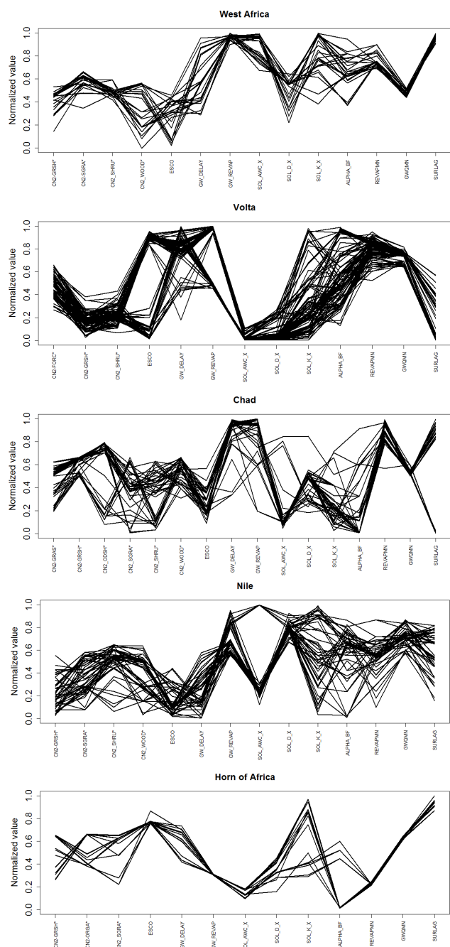
Fig. 8. Estimates of SWAT calibration parameters obtained from multi-criteria calibration (abbreviations of the land cover type: FOC – Closed deciduous forest; FORC – Closed evergreen lowland forest; FORD – Degraded evergreen lowland forest; FORS – Submontane forest; GRAS – Closed grassland; GRSH – Open grassland with sparse shrubs; ODSH – Open deciduous shrubland; OGRA – Open grassland; SAVA – Mosaic Forest/Savanna; SGRA – Sparse grassland; SHRU – Deciduous shrubland with sparse trees; WOOD – Deciduous woodland).
