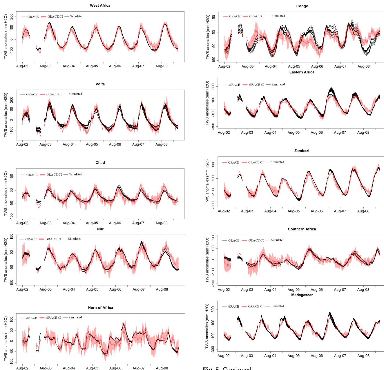
Fig. 5. Observed and zonally averaged simulated TWS variations for ten sub-continental regions (TWS-total water storage; CI-confidence).
