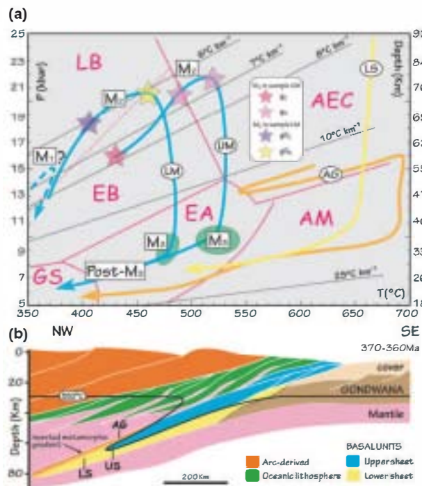
Figure 7. (a) P – T diagram showing the metamorphic paths of the Ceán Schists (LM and UM). The P – T paths for the Lower Sheet of the Malpica Tui Unit (unpublished data) and for the Agulada Unit (Arenas et al. , 1997) are also included. Metamorphic facies field abbreviations: GS, greenschist facies; EA, epidote amphibolite facies; AM, amphibolite facies; LB, lawsonite blueschist facies; EB, epidote blueschist facies and AEC, amphibole eclogite facies (Evans, 1990 (dashed line); Maruyama et al. , 1996). (b) Schematic cross-section of the subduction zone operating in the NW Iberian Massif at 370–360 Ma. US, upper sheet; LS, lower sheet; AG, Agulada Unit. Based on Martínez Catalán et al. (1996).
