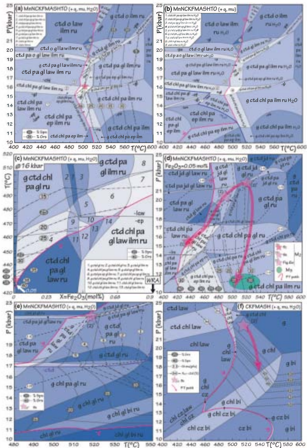
Figure 6. Sample UM [SiO 2 :68.63; TiO 2 :0.66; Al 2 O 3 :14.70; FeO: 7.68; O:0.89; MnO:0.26; MgO:3.05; CaO:0.24; Na 2 O:0.98; K 2 O:2.91] (a) P – T pseudosection with H 2 O in excess. (b) P – T pseudosection calculated for the analysed bulk-rock composition showing dehydration along the stability limit of lawsonite. (c) T – X (Fe 2 O 3 ) pseudosection calculated at 16 kbar between 420 and 520 °C; WRA original whole-rock analysis from XRF. (d) P – T pseudosection with Fe 2 O 3 = 0.05 mol %. The star (2)* is inferred from Fig. 6e. (e) P – T pseudosection calculated for the bulk-rock composition after fractionation of garnet and chloritoid. (f) P – T pseudosection calculated in the CKFMASH system for the bulk-rock composition after fractionation. The star (2)* is inferred from (e). See text and Table 1 for details.
