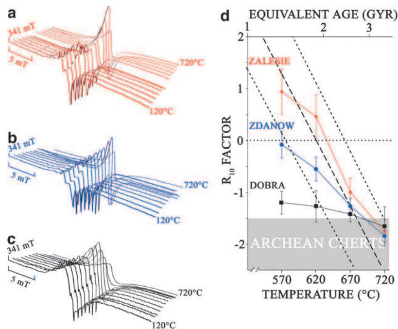
FIG. 5. Evolution of the EPR signals during step thermal treatment of (a) the Zalesie Nowe chert, (b) the Zdanow chert, (c) the Döbra chert, and (d) the calculated R_{10} factors. The correlation of R_{10} factor with age is given in dashed line with its error margin. Equivalent age is given in the upper abscissa. Color images available online at www.liebertonline.com/ast
