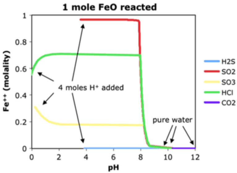
Figure 8. Aqueous concentration of free Fe ++ species during dissolution of 1 mole of FeO (the ferrous component in mineral) by fluids of various acidity. The pH of the resulting solution depends on the concentration and also the nature of the acidic reactant. The conjugate anions strongly influence the amount of the aqueous ferric specie following a general equation: \text{FeO} + \text{H}_2\text{O} + \text{HX} \rightleftharpoons a\text{Fe}^{++}_{\text{aq}} + b\text{FeX}^{-}_{\text{aq}} + c\text{FeX}_2_{\text{aq}} + d\text{FeX}_2_{\text{solid}} .
