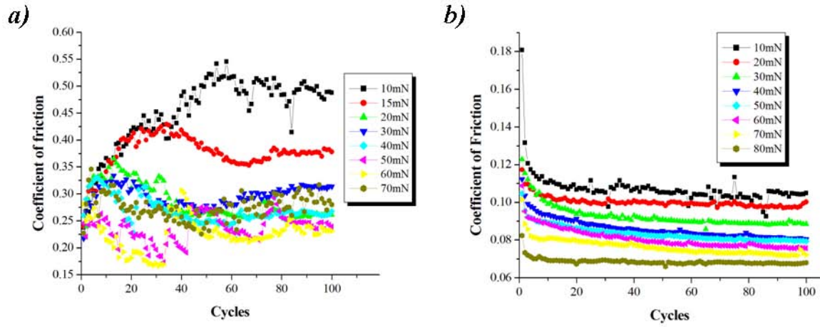
Figure 4: Evolution of the coefficient of friction with the normal load in the face-on configuration: (a) high level regime , and (b) low level regime
