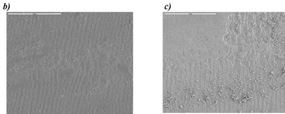
Figure 8: Tribological features in the face-on low level regime: (a) evolution of the dissipated energy with the applied normal load vs. that of high regime; (b) and (c) typical SEM views of the friction track at low (20 mN) and high normal load (70 mN), respectively (bars are 50 \mu\text{m} )
