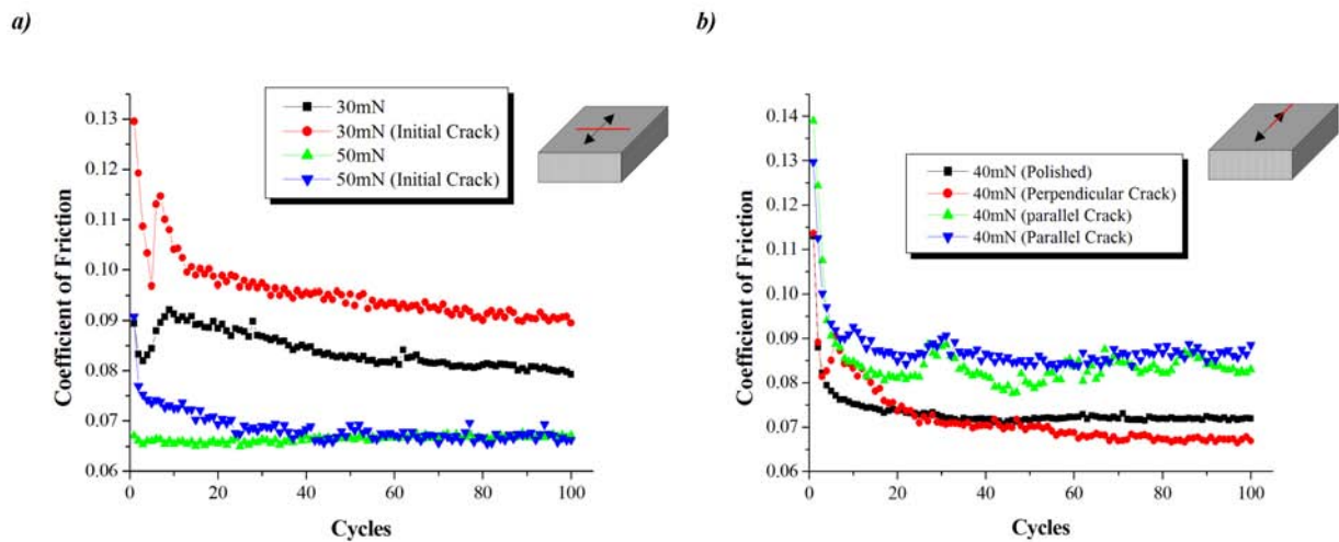
Figure 17: Influence of the presence of an initial scratch (a) perpendicular and (b) parallel to the direction of sliding on the frictional behaviour
