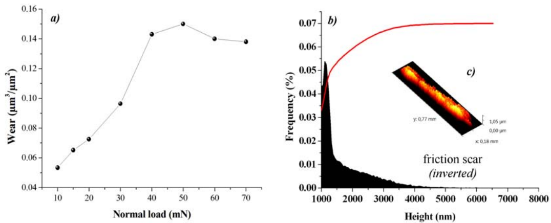
Figure 5: Wear assessment in the face-on high level regime: for each applied normal load, wear (a) is computed by integration of the height distribution histograms (b) from the topographical features of the inverted friction scar (c)
