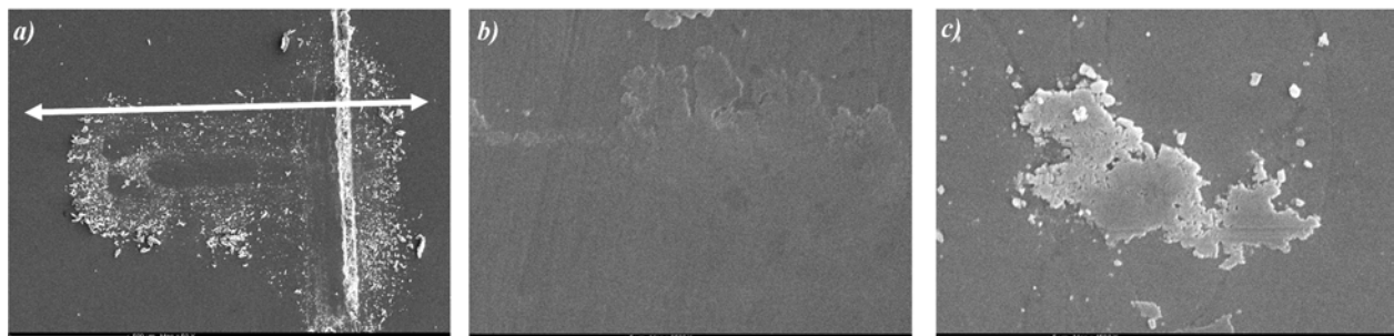
Figure 13: (a) Typical SEM views of the friction track after 100 cycles, in presence of initial scratch; (b) enlargement on the friction track (c) typical view of the discontinuous tribolayer (bar is 500 \mu\text{m} , 5 \mu\text{m} and 5 \mu\text{m} , respectively)
