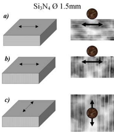
Figure 1: Various configurations of the samples: (a) face-on orientation ; (b) edge-on perpendicular to the sliding direction, and (c) edge-on parallel to the sliding direction
