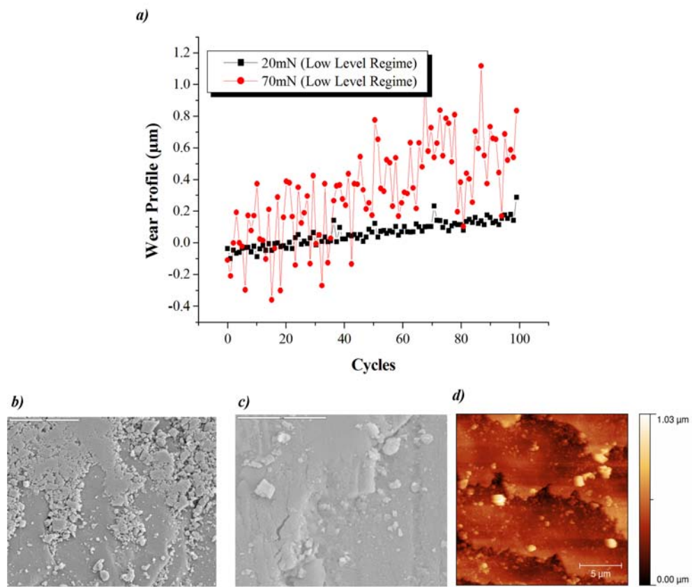
Figure 10: Wear features in the face-on low level regime: (a) in situ wear profile assessment carried out in the center of the friction track; (b) typical SEM view of the friction track; (c) and (d) typical views of the wear mechanism occurring in the face-on low level regime in SEM and AFM, respectively (bar is 5 \mu\text{m} , 2 \mu\text{m} and 5 \mu\text{m} , respectively)
