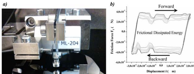
Figure 2: Nanotribological setup: (a) picture showing the two real-time measuring optical sensors (i) the horizontal one records the friction force and (ii) the vertical one records the time-dependent wear properties; (b) typical view of the friction loop allowing to compute the dissipated frictional energy, and the difference between the forward and backward friction force
