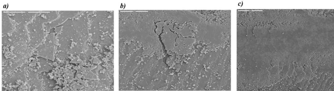
Figure 7: Typical SEM views of the friction track in the face-on high level regime: (a) at low applied normal load (20 mN – bar is 10 μm); (b and c) at high applied normal load (70 mN – bar is 10 μm and 20 μm, respectively)
