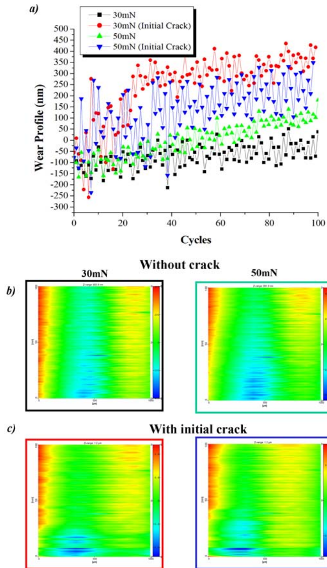
Figure 14: in situ tribological behaviour in the edge-on configuration perpendicular to the sliding direction, for two applied normal load (30 mN and 50 mN): (a) various in situ wear profiles carried out in the center of the friction track, in absence and in presence of initial scratch, respectively; Corresponding wear maps (b) in absence, and (c) in presence of initial scratch
