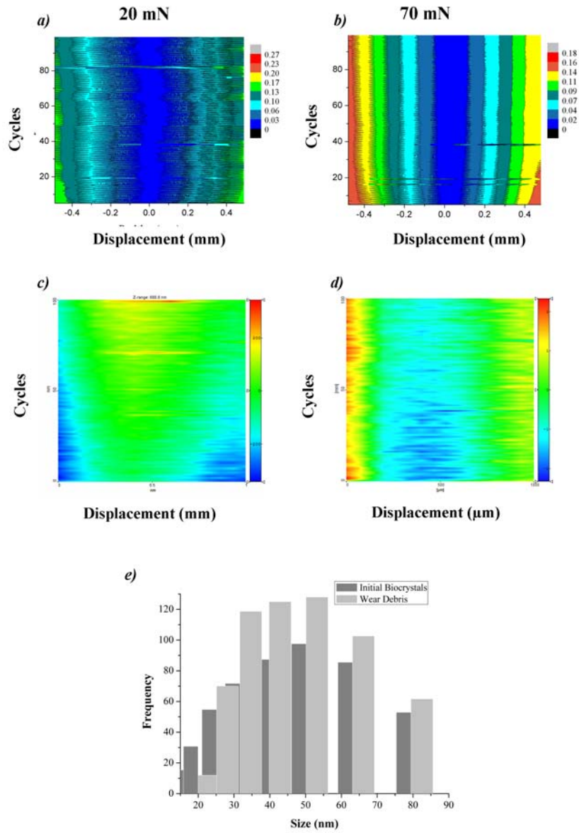
Figure 9: in situ tribological behaviour in the face-on low level regime, for two applied normal loads: (a) friction maps at 20 mN, and (b) at 70 mN; (c) wear maps at 20 mN, and (d) at 70 mN. (e) Comparison of the particles size distribution curves of wear debris with that of nanograins in the initial biocrystal
