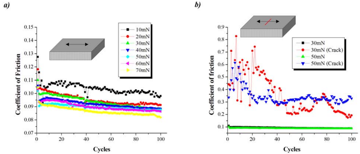
Figure 12: Evolution of the friction coefficient in the edge-on configuration perpendicular to the sliding direction (a) in absence, and (b) in presence of initial scratch
