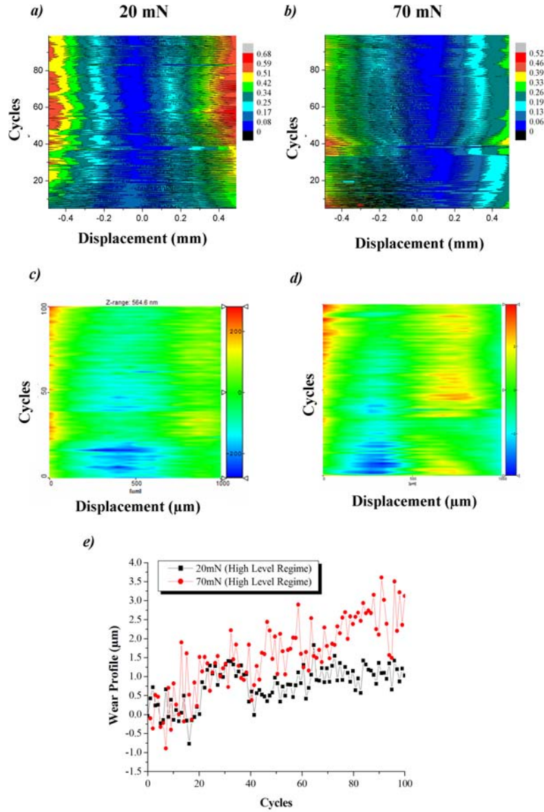
Figure 6: in situ tribological behaviour in the face-on high level regime for two applied normal loads: (a) friction maps at 20 mN, and (b) at 70 mN; (c) wear maps at 20 mN, and (d) at 70 mN; (e) corresponding in situ wear profile assessment carried out in the center of the friction track
