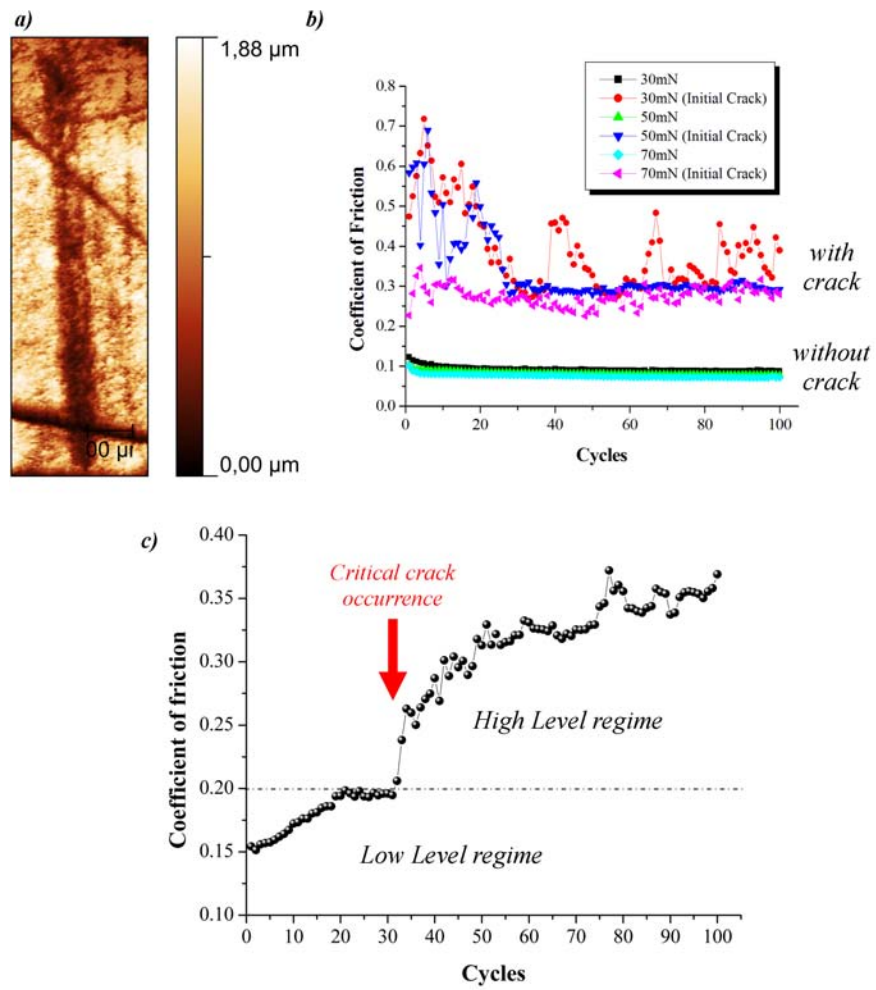
Figure 11: (a) Typical view of the friction track after sliding in the face-on high level regime ; (b) Evolution of the friction coefficient in absence and in presence of scratch;(c) example of transition from low to high level friction regime due to the occurrence of a critical crack around 35 cycles (Normal load 30 mN):
