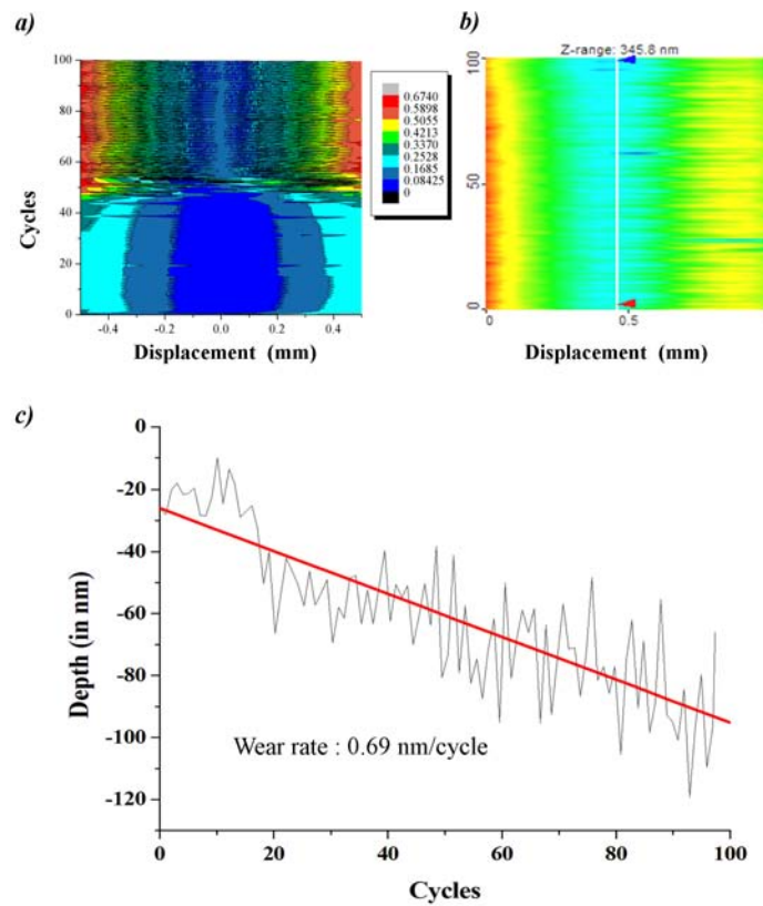
Figure 3: Typical views resulting from the in situ triboscopic approach giving simultaneously and for each cycle: (a) the evolution of the friction coefficient along the friction track ( friction map ); (b) the evolution of the time-dependent wear process and/or potential build-up of a tribolayer within the contact ( wear map ); and (c) the in situ wear rate assessment by using a classical profile analysis
