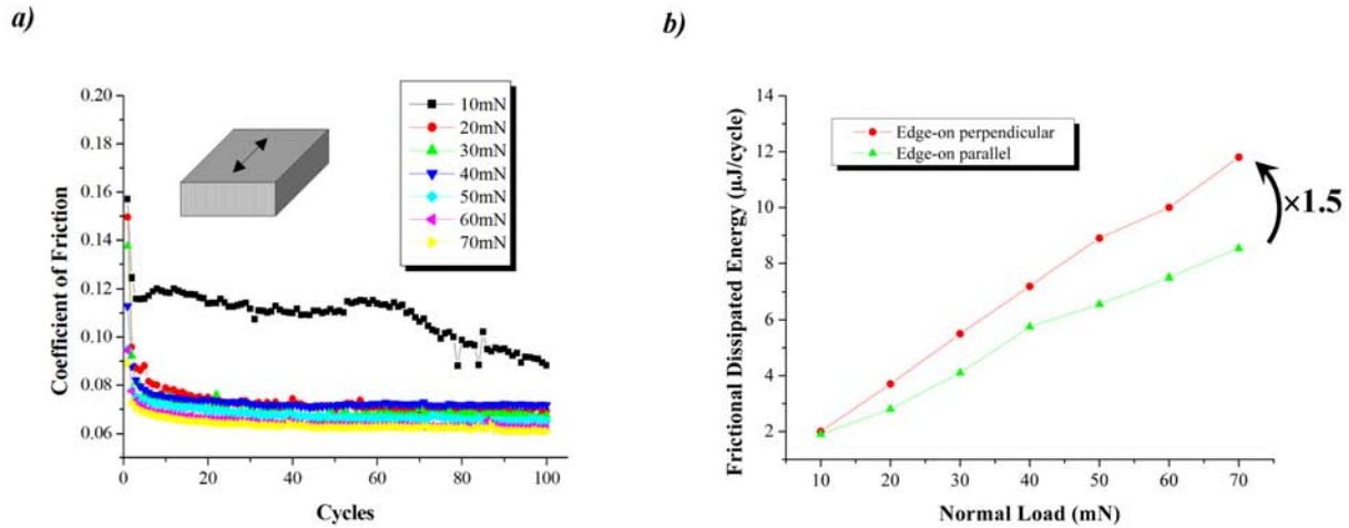
Figure 16: Frictional features in the edge-on configuration parallel to the sliding direction: (a) Evolution of the friction coefficient with the number of cycles ; (b) Evolution of the frictional dissipated energy with the applied normal load
