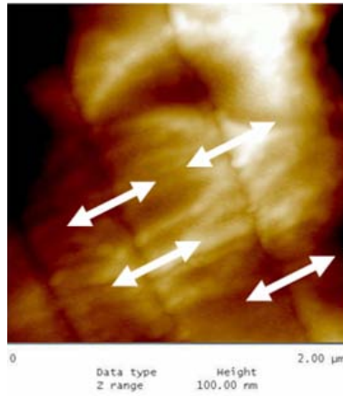
Figure 15: Effect of the vertical organic/mineral interfaces on the frictional dissipation mechanism in the edge-on configuration perpendicular to the sliding direction
