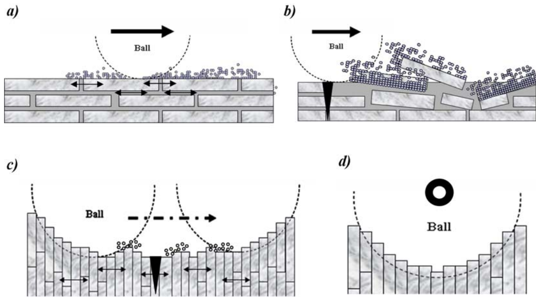
Figure 20: Various friction-induced energy dissipation ways of sheet nacre as a function of its orientation: (a) face-on low level regime; (b) face-on high level regime ; edge-on perpendicular (c) and parallel (d) to the sliding direction
