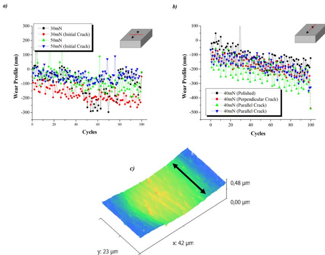
Figure 19: in situ wear profile assessments carried out in the edge-on parallel direction in absence and in presence of initial scratch (a) perpendicular and (b) parallel to the sliding direction, respectively; (c) Typical AFM view of the friction track after sliding
