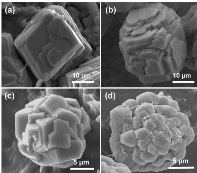
Figure 4. SEM images of magnified \text{CaCO}_3 crystals grown in silk fibroin hydrogel with varying silk fibroin concentrations (wt. %): (a) 5%, (b) 10%, (c) 15%, and (d) 25%.
