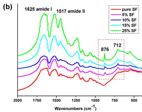
Figure 5. XRD patterns (a) and FTIR spectra (b) of the pure silk fibroin gel and silk fibroin/ \text{CaCO}_3 hybrids.
