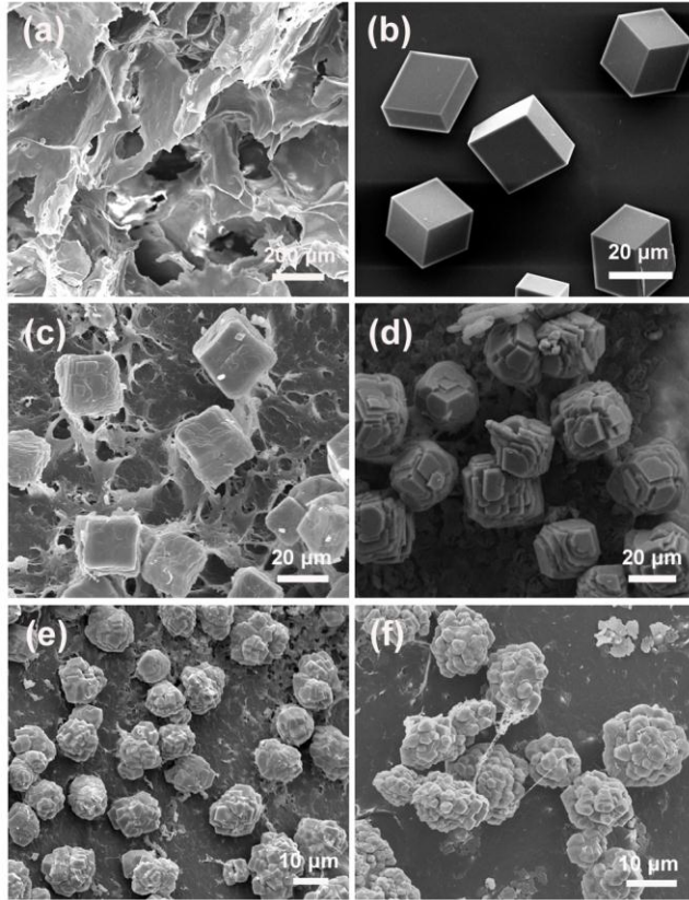
Figure 3. SEM images of the pure silk fibroin gel (a), \text{CaCO}_3 crystals grown without silk fibroin gels (b) and \text{CaCO}_3 crystals grown in the gels with varying silk fibroin concentrations (wt. %): (c) 5%, (d) 10%, (e) 15%, and (f) 25%.
