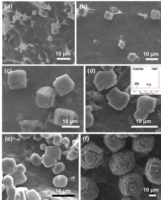
Figure 6. SEM images of crystallization process of CaCO 3 crystals in 10% silk fibroin hydrogel at different interval: (a) 5 min, (b) 10 min, (c) 2 h, (d) 6 h, (e) 8h, and (f) 12 h. Inset shows polymorph of the sheet-like crystal by micro-Raman spectra.
