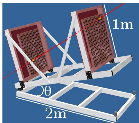
Fig. 2. Schematic view of a muon telescope equipped with two matrices with 16 \times 16 pixels.
