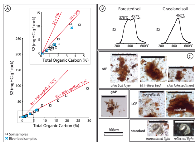
Fig. 5. Rock-Eval results (A) of soil and riverbed samples are represented by the diagram S2 vs. (%). The two linear domains of the hydrogen index ( HI = 750 and HI = 300 \text{ mgHC g}^{-1} \text{ TOC} ) corresponding to algal and terrestrial poles, respectively, are represented. S2 curve (B) from Rock Eval analysis on superficial layers from forested and grassland soils are also presented. Thermal cracking of the hydrocarbon compounds are represented by the temperature. Organic particles identified by quantitative organic petrography are illustrated in (C): rAP in soil layers, riverbeds and lacustrine sediment; gAP; LCF non-altered or oxidized; and the standard added in transmitted and reflected light modes.
