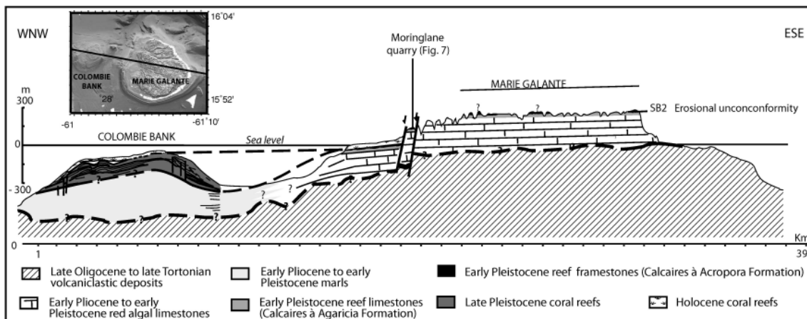
FIG. 10. – Simplified cross-section from Marie-Galante to Colombie bank. Onshore, data are from the geological map of Marie-Galante [Bouysse et al. , 1993] and personal observations. Offshore, the geology of the Colombie bank was interpreted from the seismic profil K08_73 (fig. 8A) and K08_10 of the KaShallow 1 cruise.
