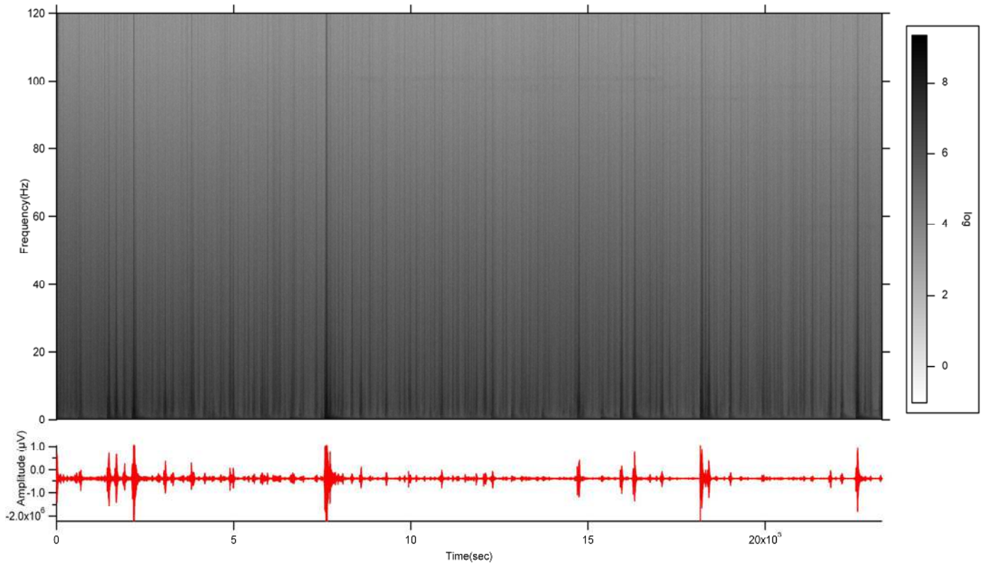
Figure 9 Record example of 6.5 hours of data, collected south of Azores islands near the mid-Atlantic ridge. Time series is in red, spectrogram in greyscale.
