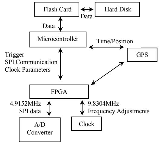
Figure 8 Block diagram of the acquisition system.
