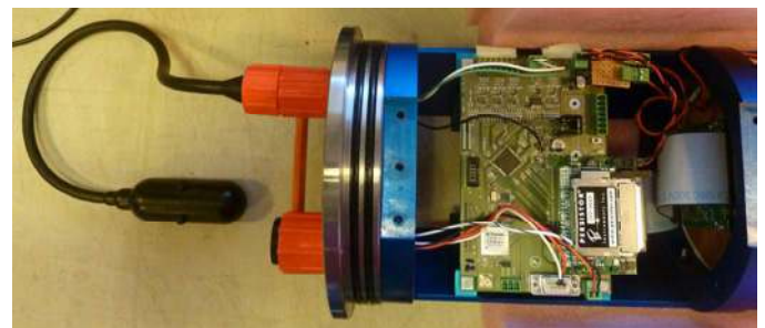
Figure 6 Hydrophone electronic board and sensor.
