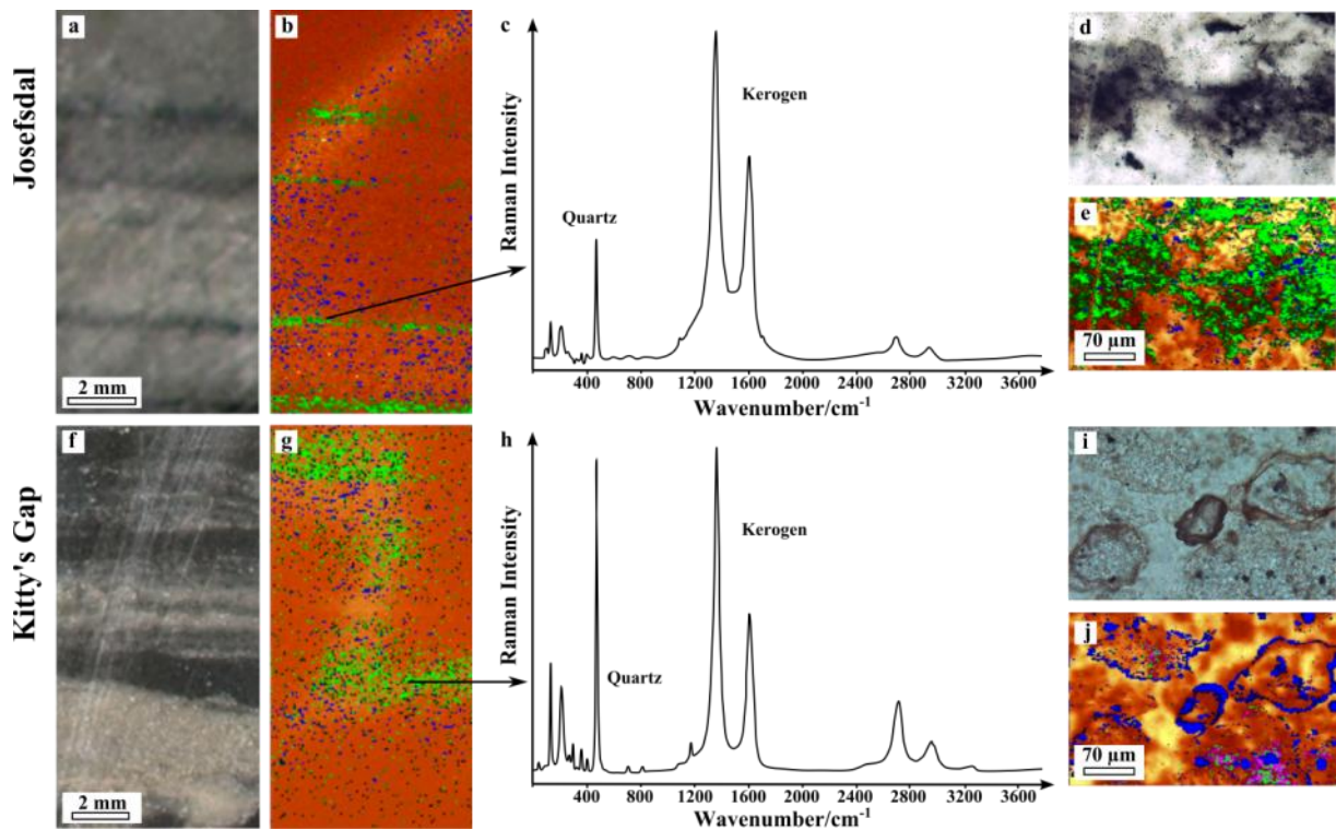
Figure 6. Chert samples from (a-e) Josefsdal, Barberton Greenstone Belt, South Africa, and (f-j) Kitty's Gap, Pilbara, Australia. (a,f) Photography of the cut and polished surfaces and (b,g) corresponding Raman maps, where carbonaceous matter (kerogen) appears green, anatase ( \text{TiO}_2 ) blue and quartz orange. These Raman maps allow rapid detection of areas of interest which can be targeted for further analyses with higher resolution spectral (c,h) and imaging (optical (d,i) and Raman (e,j)) techniques.
