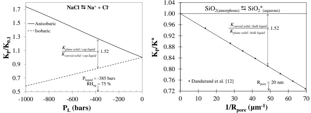
Fig. 2. Isobaric and anisobaric contexts illustrated for (a) NaCl solubility as a function of capillary pressure; (b) amorphous silica solubility as a function of pore radius (compared to experiments from [12]).
