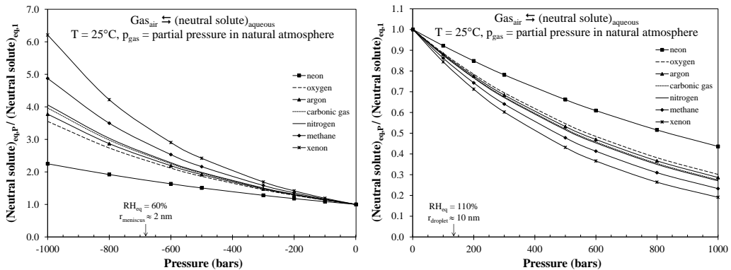
Fig. 1. Gases solubility ratio between capillary and bulk water and (a) concave-curved capillary water; (b) convex-curved droplet.
