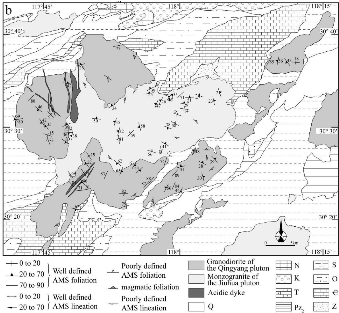
Figure 11 Magnetic foliation (a) and lineation (b) maps of the granitic rocks in the Qingyang-Jiuhua massif. Q: Quaternary, N: Tertiary, K: Cretaceous, T: Triassic, Pz 2 : upper Paleozoic, S: Silurian, O: Ordovician, ε: Cambrian, Z: Sinian.
