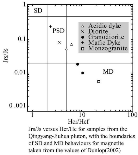
Figure 7. J_{rs}/J_s versus H_{cr}/H_c diagram from measured samples of the Qingyang-Jiuhua massif to define the magnetite size. J_{rs} : remanence, J_s : saturation remanence, H_{cr} : coercivity of remanence, H_c : coercivity, SD: single domain, PSD: pseu-single domain, MD: multi-domain, respectively.
