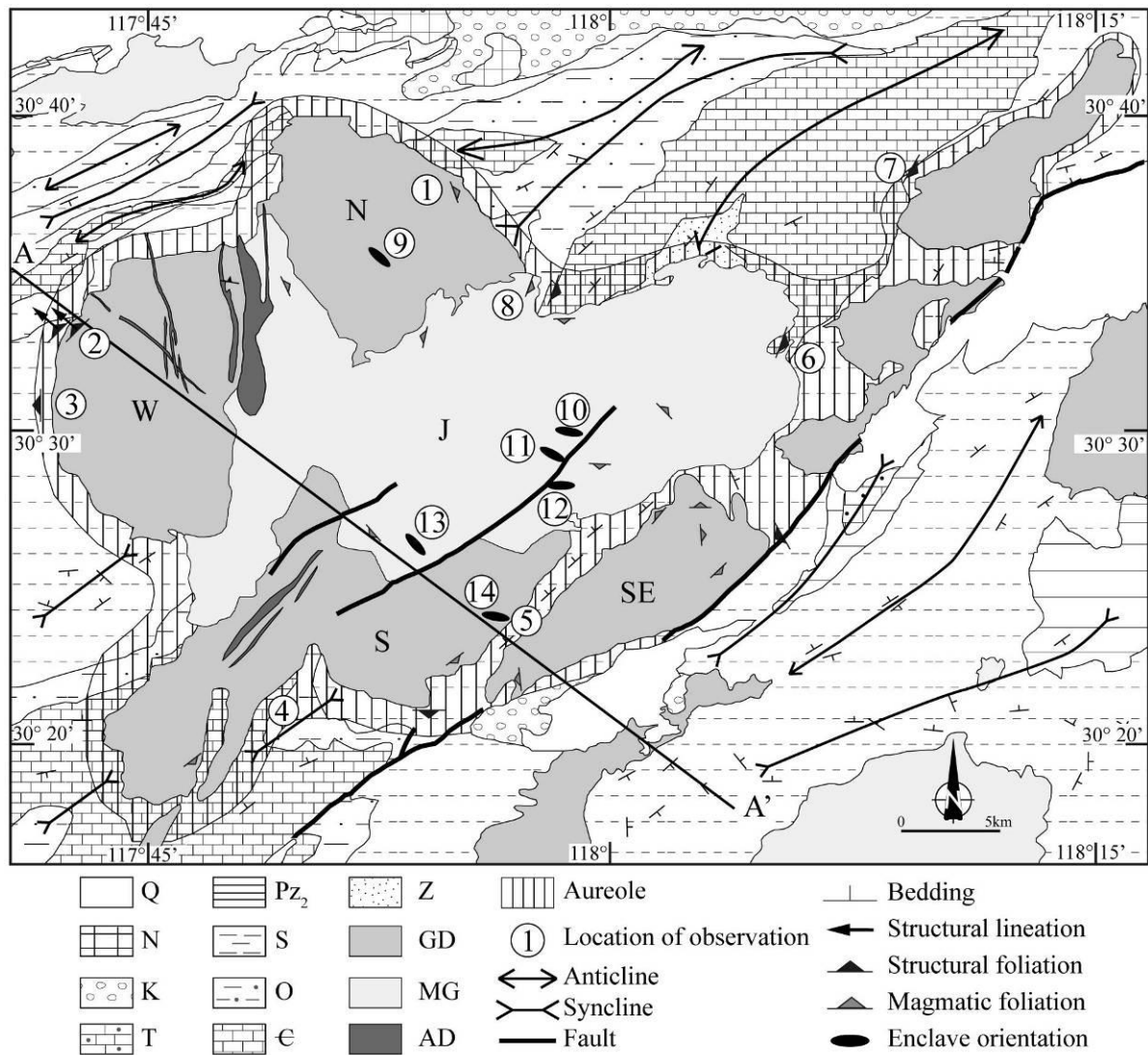
Figure 2. Simplified geological map of the Qingyang-Jiuhua massif area. Q: Quaternary, N: Tertiary, K: Cretaceous, T: Triassic, S: Silurian, O: Ordovician, Є: Cambrian, Z: Sinian, GD: Granodiorite of the Qingyang pluton, MG, Mongzogranite of the Jiuhua pluton, AD: Acidic dyke, J , N , W , S and SE represent for the Jiuhua pluton, the northern, western, southern and southeastern subplutons of the Qingyang pluton, respectively.
