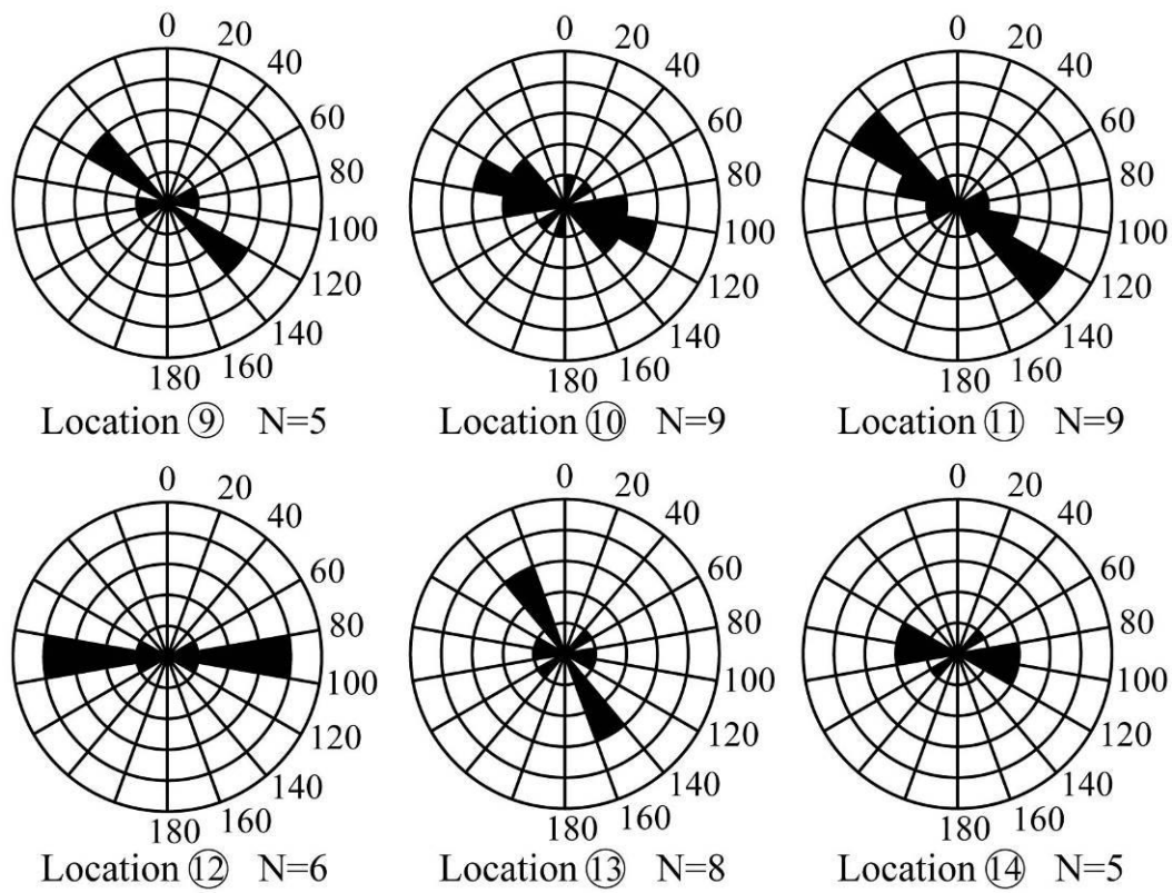
Figure 4. Preferred orientation of microgranitoid enclaves (Sample locations shown in Figure 2).
