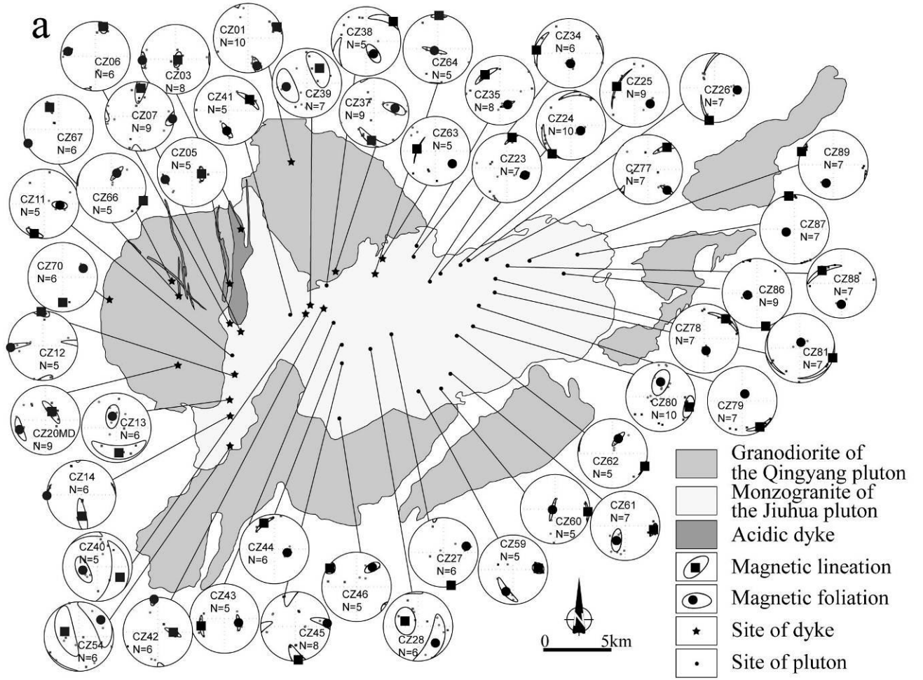
Figure 9 a and b present the equal area lower hemisphere projection of each site from the dykes and the monzogranite of the Jiuhua pluton as well as the granodiorite of the Qingyang pluton respectively. Squares and circles stand for K1 (magnetic lineation) and K3 (pole of magnetic foliation), respectively. Small grey and larger black squares or circles represent individual specimen and site-mean direction, respectively with their confidence ellipses at 95% level.
