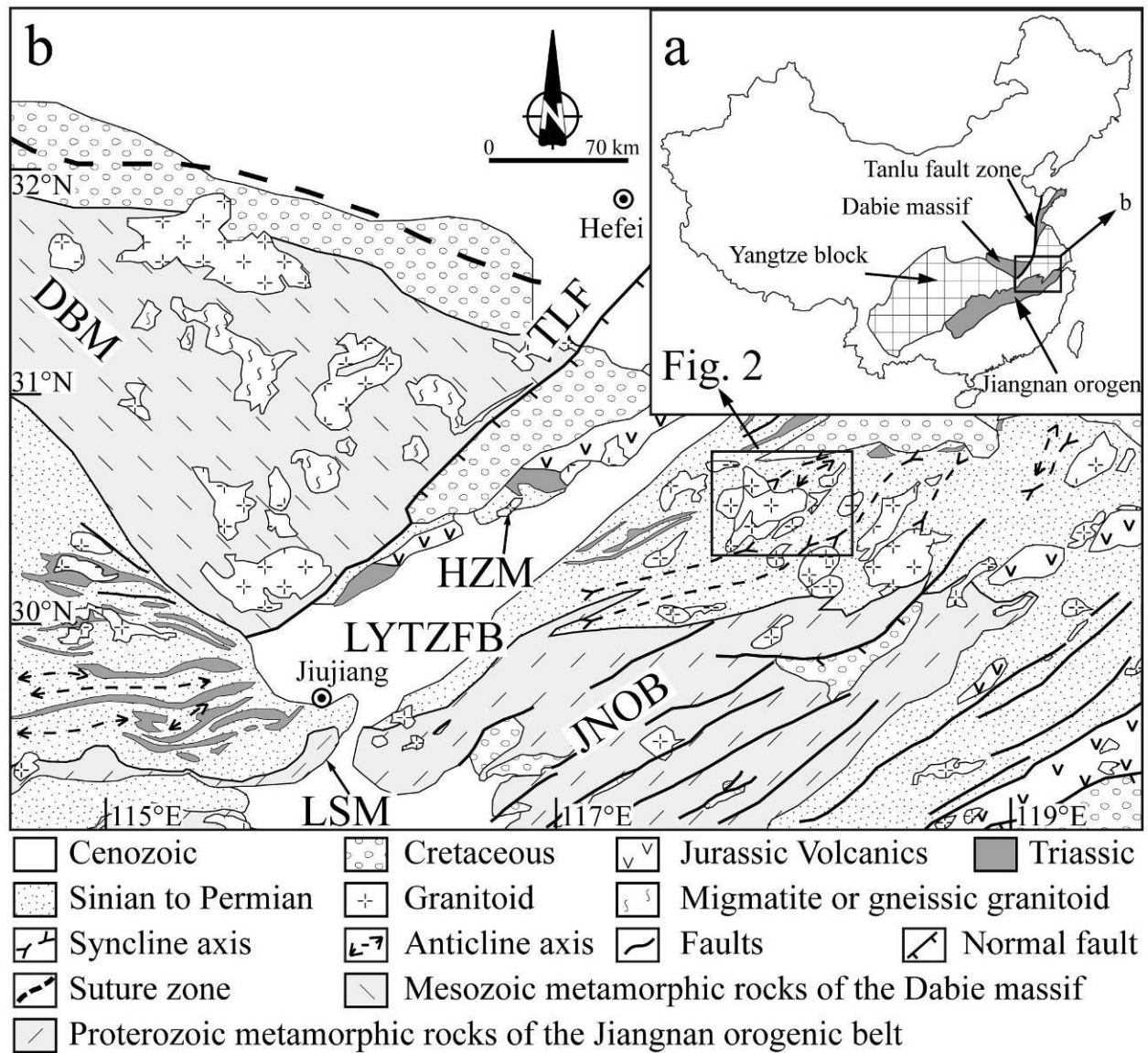
Figure 1. Regional geological map. DBM: the Dabie massif, LYZFB: the Lower Yangtze fold belt, JNOB: the Jiangnan orogenic belt, TLF: the Tanlu fault, HZM: the Hongzhen massif.
