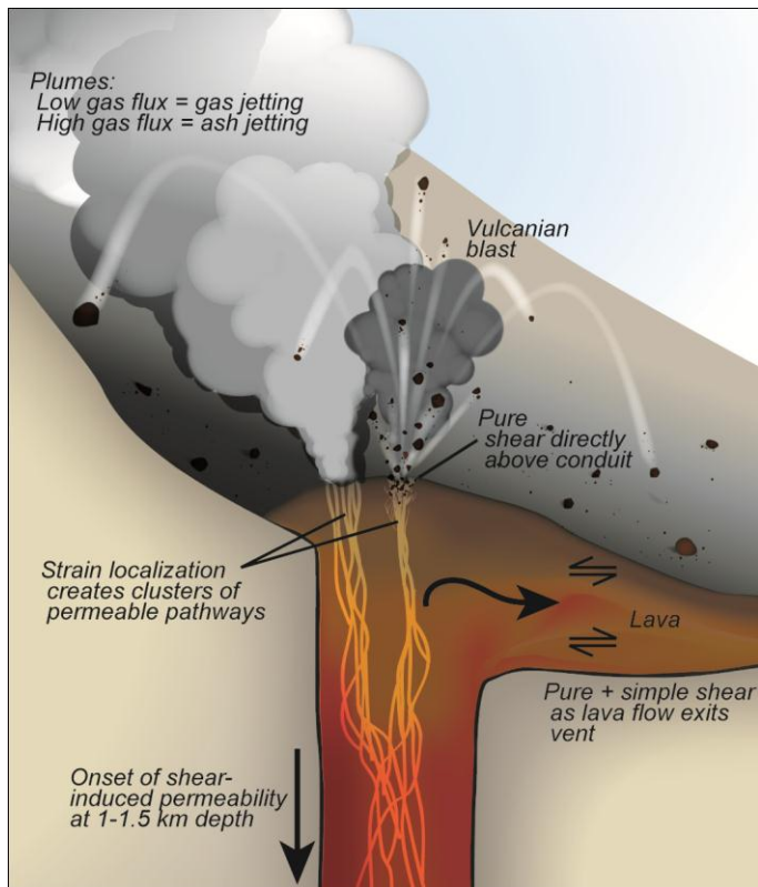
Fig. 10. Cartoon (not to scale) of cross-sectional view through the shallow vent and upper conduit of Cordón Caulle during the observed hybrid activity.
