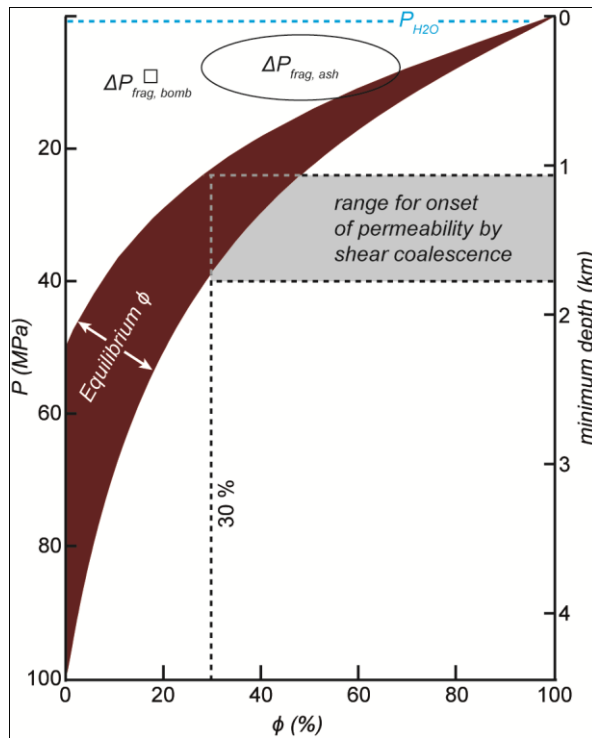
Fig. 8. Pressure ( P ) versus porosity ( \phi ) for Cordón Caulle magma. Pressures also expressed as minimum depths using density of dense magma, \rho_m = 2300 \text{ kg m}^{-3} . Envelope of equilibrium \phi calculated following Burgisser and Gardner (2005), for the shallowest (50 MPa) and deepest (100 MPa) Cordón Caulle magma storage depths experimentally determined by Castro et al. (2013). Zero porosity at storage is assumed, as is \text{H}_2\text{O} solubility following Henry's law, with constant \kappa = 3.5 \times 10^{-6} \text{ kg}^{-0.5} \text{ m}^{-0.5} \text{ s} of a generic rhyolite (Newman and Lowenstern, 2002). Range of depths at which equilibrium porosity reaches 30% may be depth at which shear coalescence becomes important (Okumura et al., 2009), and thus may mark the depth to which sub-volcanic degassing structures penetrate. Also indicated are the ranges of \Delta P_{frag} versus \phi for the ash and bombs (Table 1), and the equilibration pressure of pyroclasts as indicated by their residual \text{H}_2\text{O} contents ( P_{\text{H}_2\text{O}} ; equivalent for ash and bomb at scale of figure). Note that P_{\text{H}_2\text{O}} \ll than the pressures suggested by equilibrium \phi envelope indicates that open system degassing has occurred, and P_{\text{H}_2\text{O}} < \Delta P_{frag} indicates that fragmentation was not primarily by bubble overpressure.
