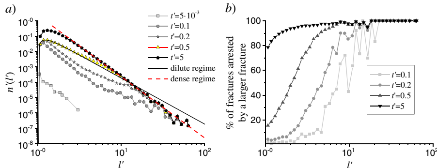
Figure 5. (a) Evolution with time of the length distribution with mode A and other parameters same as in Figure 4. (b) Percentage of arrested fractures.
