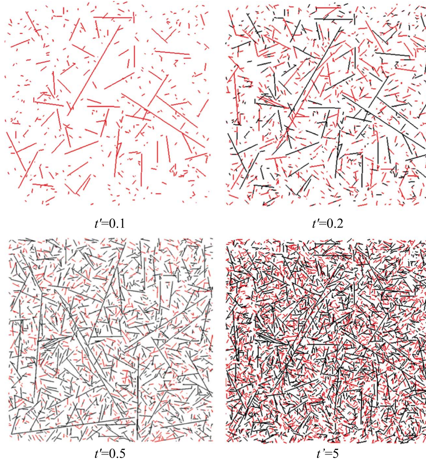
Figure 8. Illustration of the DFN generation and evolution (same as Figure 5). 2D trace map views—(xy) plane, z=0 —from a 3D DFN generation with the following parameters: a power-law nuclei distribution with b=5 and l_N=10^{-2} , a nucleation rate \dot{n}_N = 19 , a growth law with C=1 and a=3 , and a system size of length L=1 . The fractures generated between the previous and the current time steps are displayed in red.
