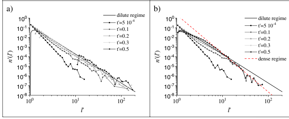
Figure 9. Evolution with time of the length distribution with no nucleation rate. All the 65,571 nuclei are present at the simulation start; this number is the same as in the case with nucleation rate for t' = 0.5 (Figure 5). Other parameters are the same as in Figure 5. (a) Model with no arrest conditions (freely growing fractures). (b) Model with mode A arrest rule.
