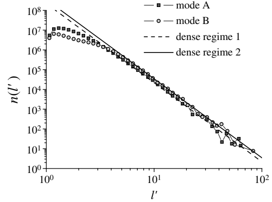
Figure 10. Length distribution for mode A and mode B UFM. Generation parameters are similar to Figure 5 and final mass density d_m' = d_m \cdot l_0 equal to 0.9.
