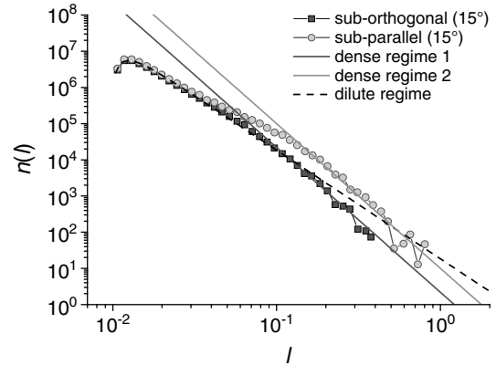
Figure 12. DFN pole orientation distribution influence on the DFN structure and UFM dense density term.
