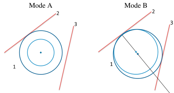
Figure 2. Illustration of the two different arrest rules. (Left) Mode A. (Right) Mode B. Fractures 2 and 3 are fixed. Fracture 1 is drawn at two different stages: light blue for the first stage where the fracture is still growing; dark blue for the second stage corresponding to the point where fracture stops growing. See text for details.
