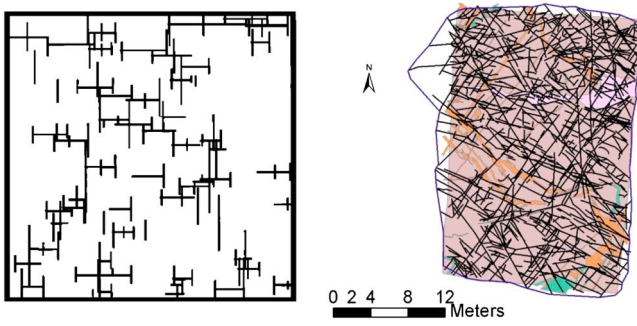
Figure 1. Fracture networks obtained from numerical simulations [Renshaw, 1996] and mapped from granitic outcrop (Forsmark, Sweden) [SKB, 2004a].
