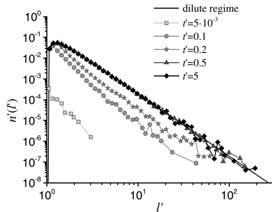
Figure 4. Evolution with time of the length distribution of the freely growing model without arrest. The parameters for the simulations are a power-law nuclei distribution p_N(l) with b = 5 and l_N = 10^{-2} , a nucleation rate \dot{n}_N = 19 , a growth law with C = 1 and a = 3 , and a system size L = 1 .
