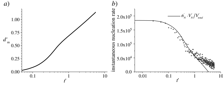
Figure 7. Evolution of (a) network density and (b) instantaneous nucleation rate with dimensionless time t' .
