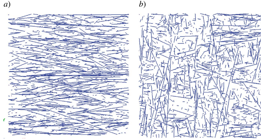
Figure 11. 2D trace map views of 3D DFNs with (a) one single set and (b) three orthogonal fracture sets.
