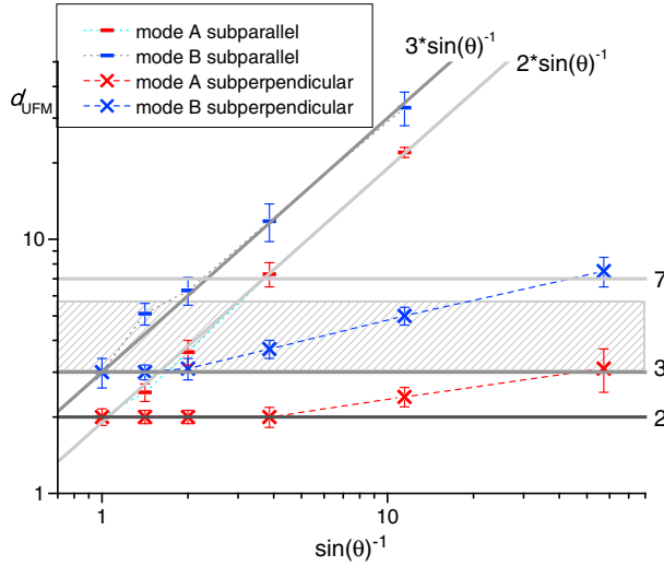
Figure 13. Evolution of the UFM density d_{\text{UFM}} as a function of the angular variability \theta (see text).
