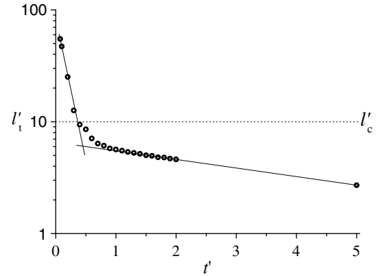
Figure 6. Evolution of the limit of the UFM regime (i.e., the smaller fracture length l_t that follows the UFM distribution) with dimensionless time t' .
