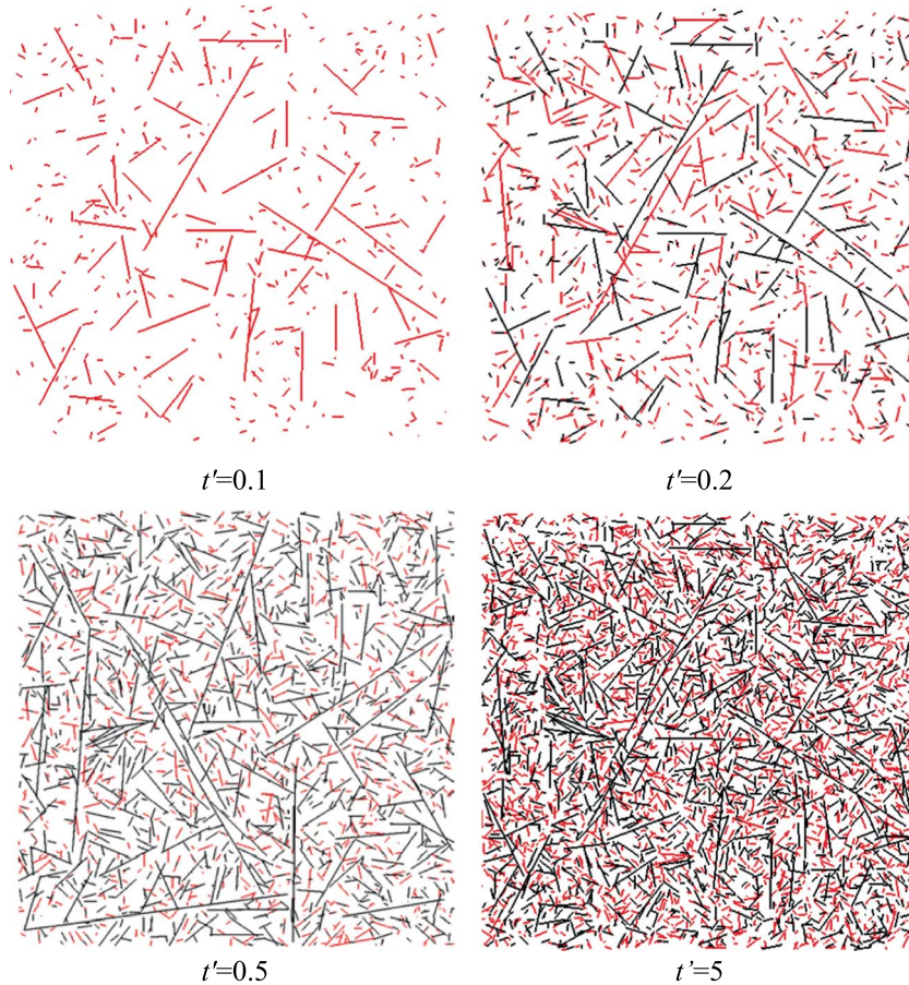
Figure 8. Illustration of the DFN generation and evolution (same as Figure 5). 2D trace map views—( xy ) plane, z = 0 —from a 3D DFN generation with the following parameters: a power-law nuclei distribution with b = 5 and l_N = 10^{-2} , a nucleation rate \dot{n}_N = 19 , a growth law with C = 1 and a = 3 , and a system size of length L = 1 . The fractures generated between the previous and the current time steps are displayed in red.
