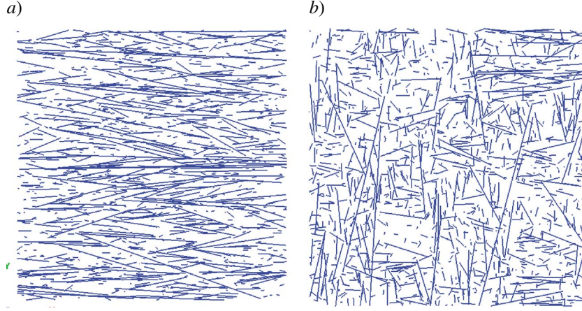
Figure 11. 2D trace map views of 3D DFNs with (a) one single set and (b) three orthogonal fracture sets.
