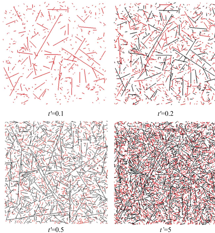
Figure 8. Illustration of the DFN generation and evolution (same as Figure 5). 2D trace map views—(xy) plane, z = 0 —from a 3D DFN generation with the following parameters: a power-law nuclei distribution with b = 5 and l_N = 10^{-2} , a nucleation rate \dot{n}_N = 19 , a growth law with C = 1 and a = 3 , and a system size of length L = 1 . The fractures generated between the previous and the current time steps are displayed in red.
