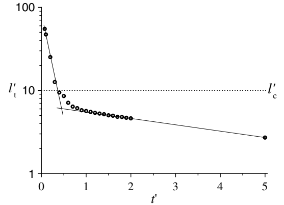
Figure 6. Evolution of the limit of the UFM regime (i.e., the smaller fracture length l_t that follows the UFM distribution) with dimensionless time t' .
