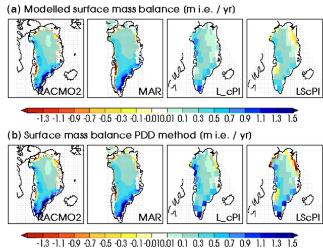
Fig. 4. (a) Climatological annual mean surface mass balance modelled on Greenland, from left to right for the regional models RACMO and MAR, the LMDZ reference simulation (LcPI) and LMDZ-SISVAT with the new snow scheme (LScPI). (b) as in (a), but for SMB computed with the PDD method ( \text{m i.e. yr}^{-1} ).
