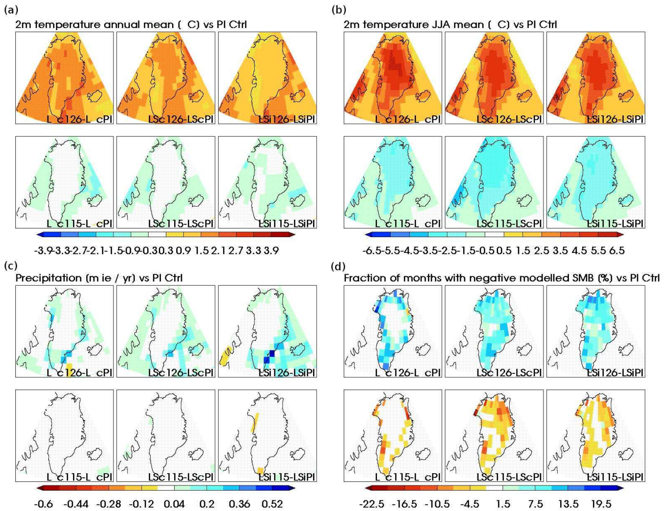
Fig. 6. (a) Climatological annual mean 2-m temperature anomaly vs. preindustrial simulation (°C) in Greenland for Eemian (top rows), and glacial inception (bottom row) simulations, in standard LMDZ (left panels) and LMDZ-SISVAT with constant climatological (centre panels) and varying (right panels) lower boundary conditions. (b) as in (a), but for climatological mean boreal summer (JJA) temperature (°C). (c) as in (a), but for climatological annual mean precipitation (m.i.e. yr -1 ). (d) as in (a), but for annual mean fraction of months with negative modelled surface mass balance.
