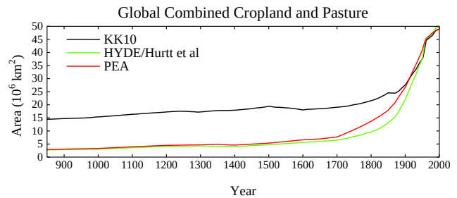
Fig. 1. Global combined cropland and pasture area in the “Kaplan and Krumhardt 2010” (KK10), Pongratz et al. (2008) (PEA) and the extended HYDE 3.1 (Hurt et al., 2009; Klein Goldewijk et al., 2011) datasets.
