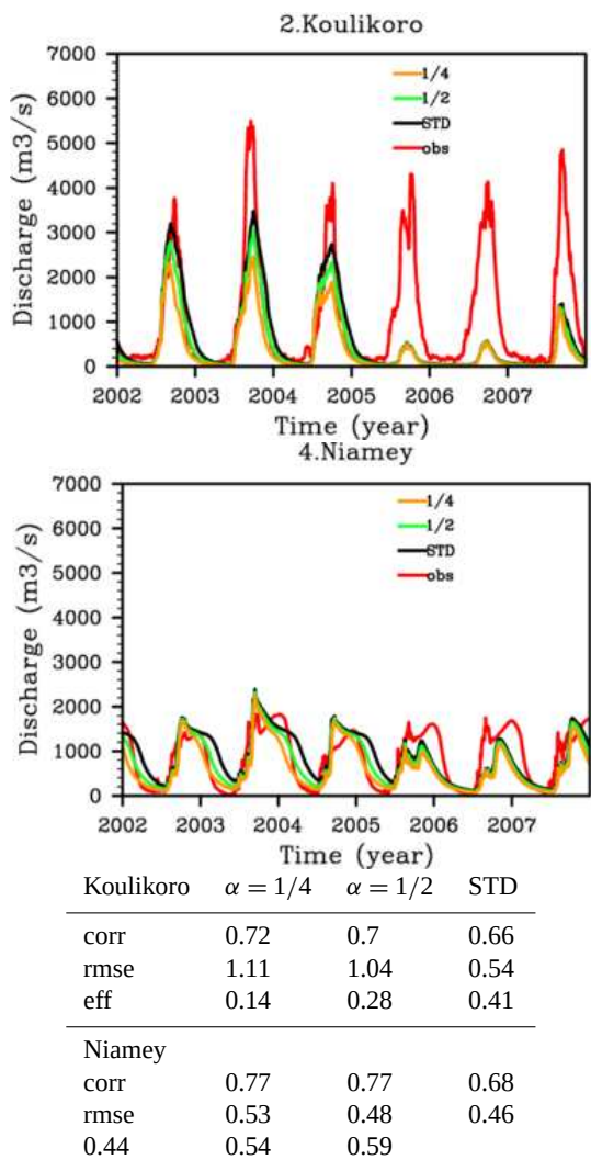
Fig. 17. Impact of aquifer distribution factor \alpha on the discharge (TRMM is used as forcing). The standard run stands for the simulation AQ-F with standard parameters (used for the simulations in previous sections).
