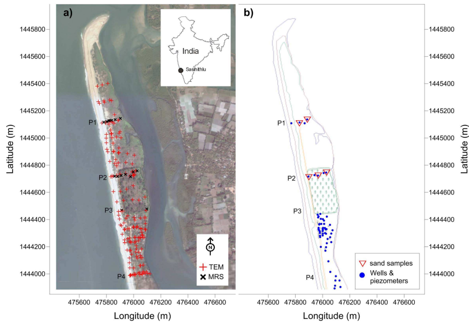
Fig. 3. Location of Sasihithlu barrier and measurements. (a) Geophysical measurements (including pre and post monsoon time lapse). (b) Hydrological measurements.
